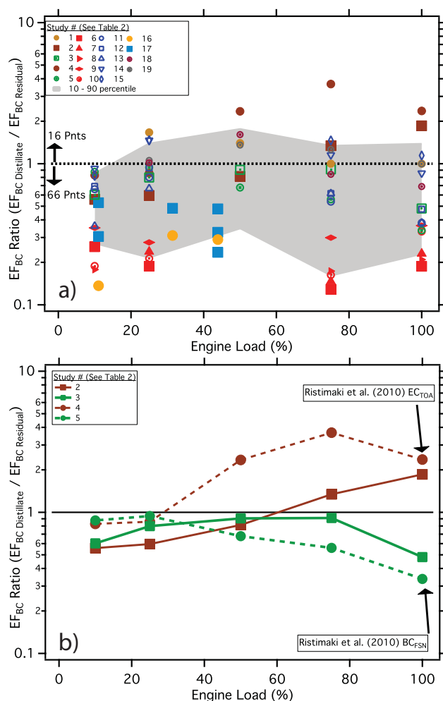
Fig. 6. (a) The change in EF_{BC} as fuel quality improves (as a ratio between EF_{BC} -Distillate and EF_{BC} -Residual). 10th–90th percentile range of data shown as shaded region, (b) Illustration of measurement inconsistency.
