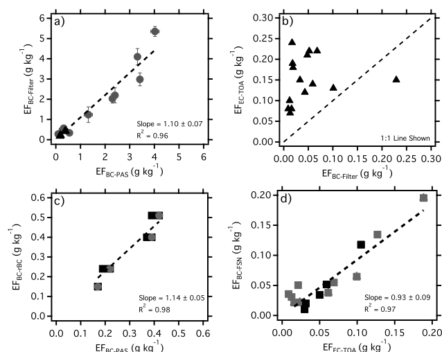
Fig. 1. Comparison of emission factors from marine diesel engines. (a) EF BC-PAS and EF BC-Filter from Lack et al. (2009) (circles) and Cappa et al. (2012) (triangles), (b) EF BC-Filter and EF EC-TOA from Petzold et al. (2011a), (c) EF BC-rBC and EF BC-PAS from Cappa et al. (2012) and (d) EF EC-TOA and EF BC-FSN from Ristimäki et al. (2010). Linear regression fit shown by dashed line in (a) , (c) and (d) . 1:1 line shown by dashed line in (b) .
