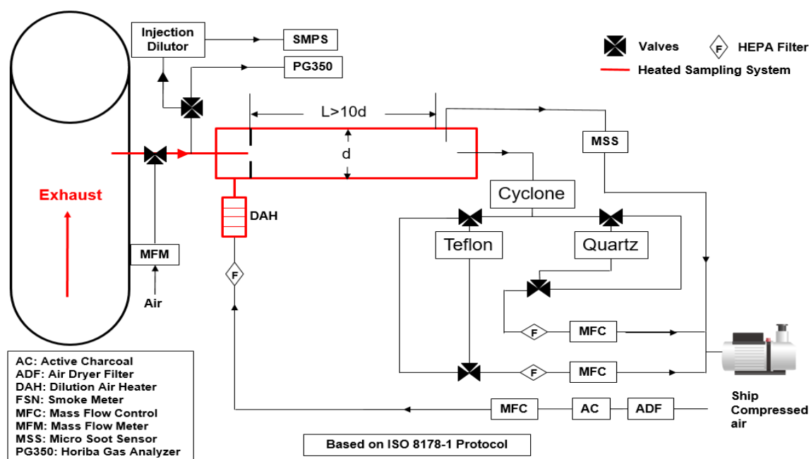
Figure 2-6 Schematic of the dilution sampling system
