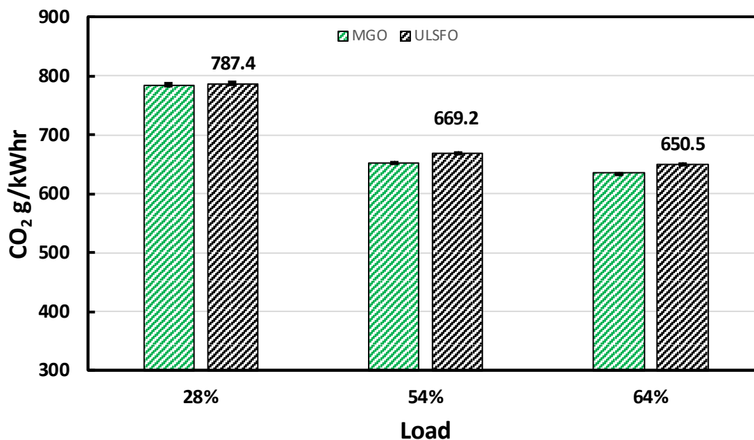
Figure 3-8 CO 2 Emissions for the AE in g/kWhr
