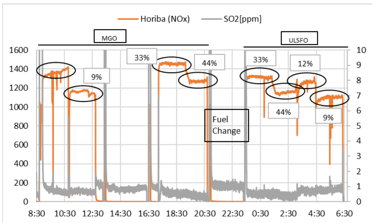
Figure F-25 Measured SO 2 soot and NO x emissions for the ME MGO and ULSFO
