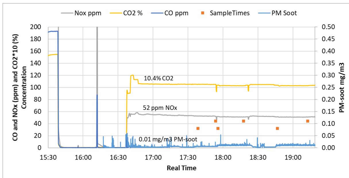
Figure F-26 Measured CO, CO2 and NO x emissions for the Auxiliary boiler MGO fuel 60% load
