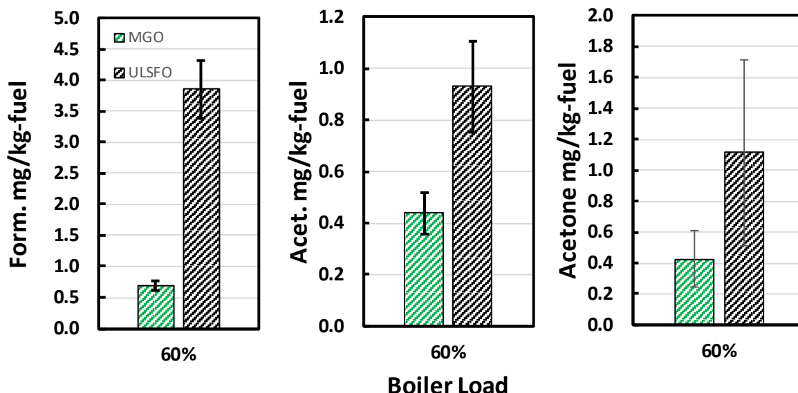
Figure 3-20 BC fuel specific toxic emissions for the auxiliary boiler in mg/kg-fuel
