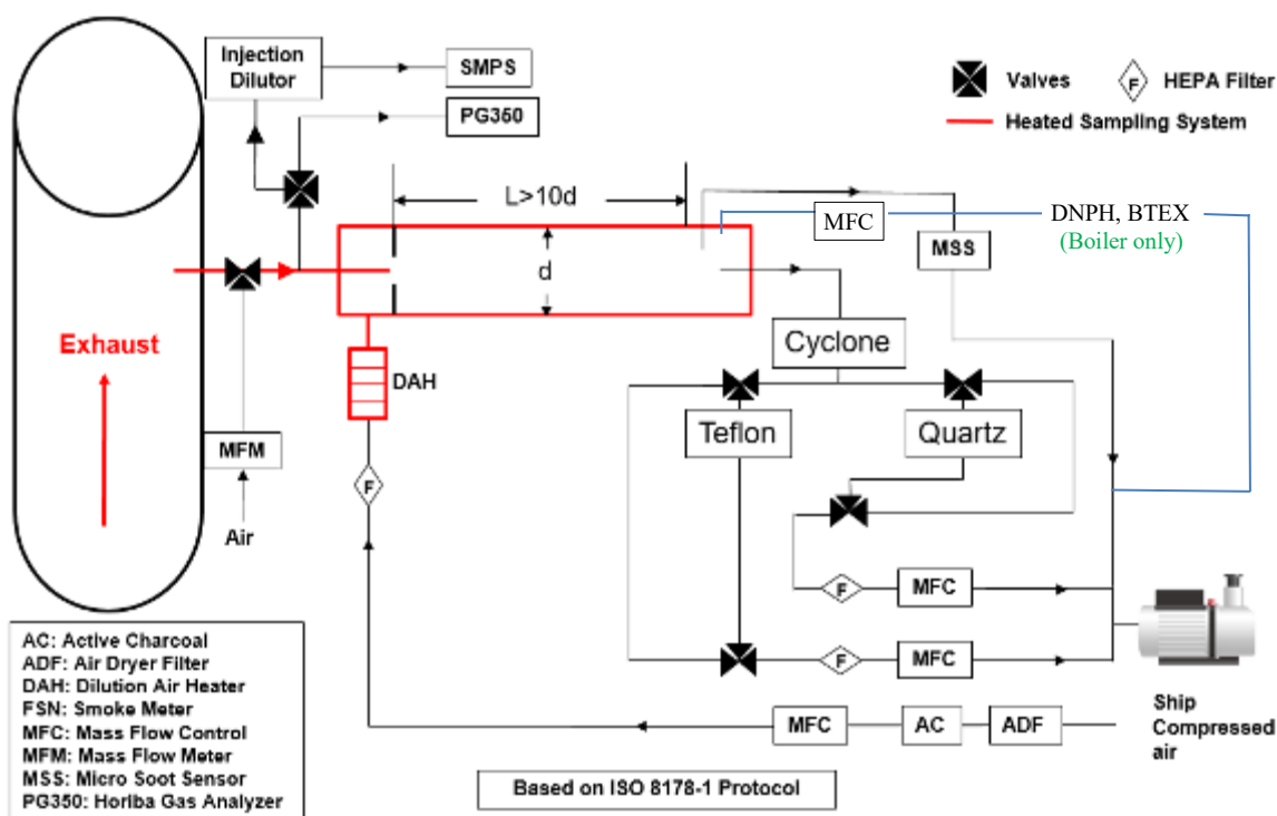
Figure 2-5 Schematic of the dilution sampling system
