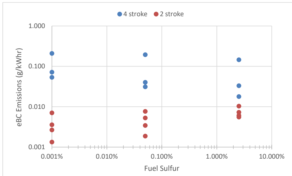
Figure 3-23 eBC (PM EC ) emissions by % load, fuel, and engine type (g/kWhr): log, log
