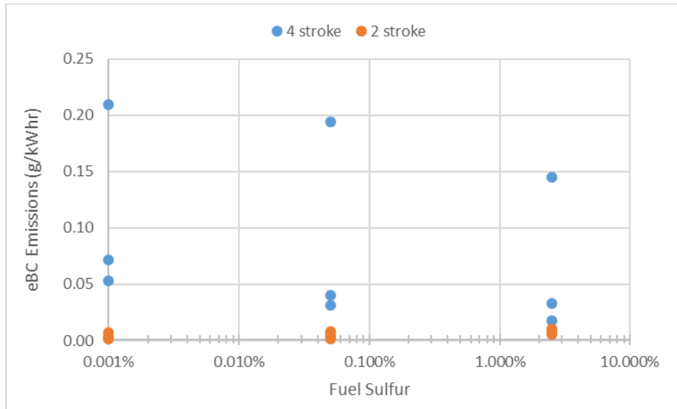
Figure 3-22 eBC (PM EC ) emissions by % load, fuel, and engine type (g/kWhr): linear, log
