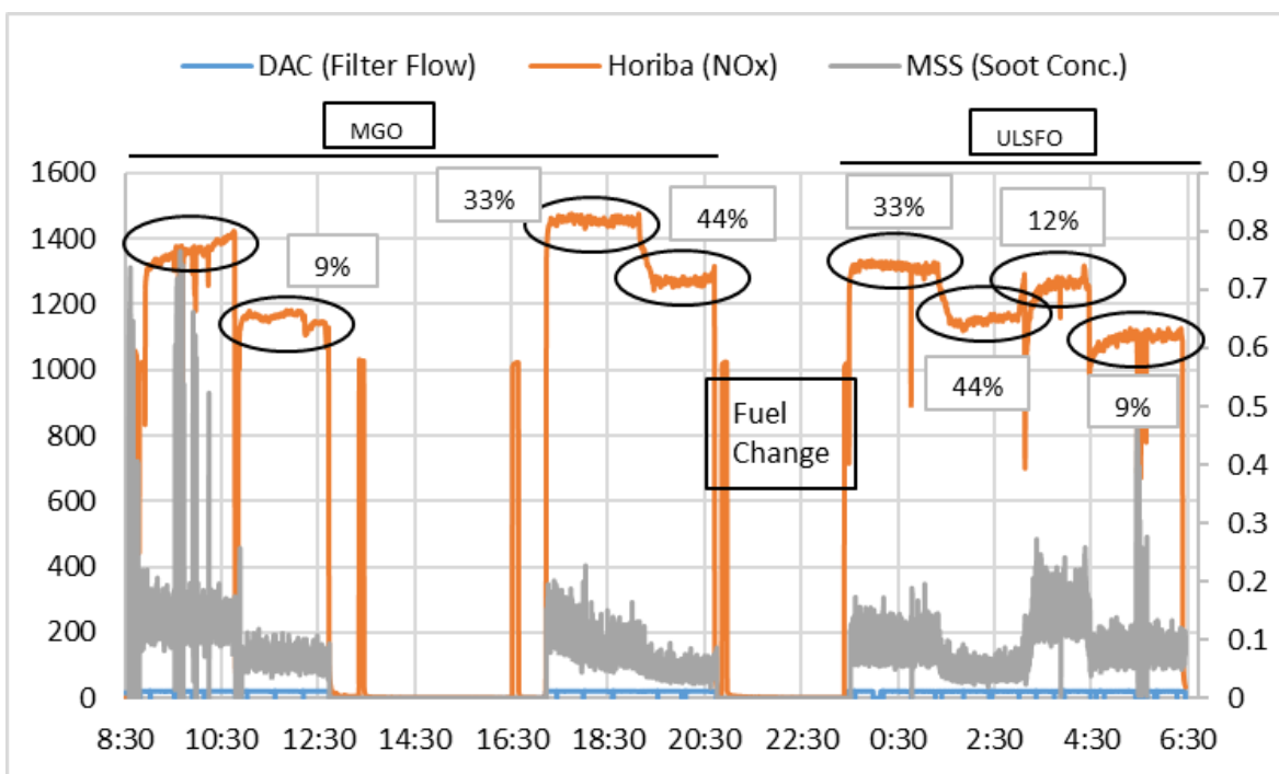
Figure F-24 Measured MSS soot and NO x emissions for the ME MGO and ULSFO
