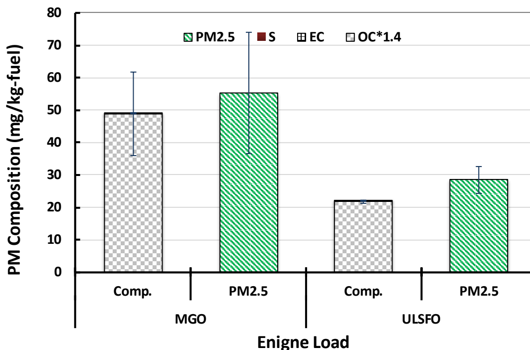
Figure 3-14 PM composition emissions for the auxiliary boiler in mg/kg-fuel
