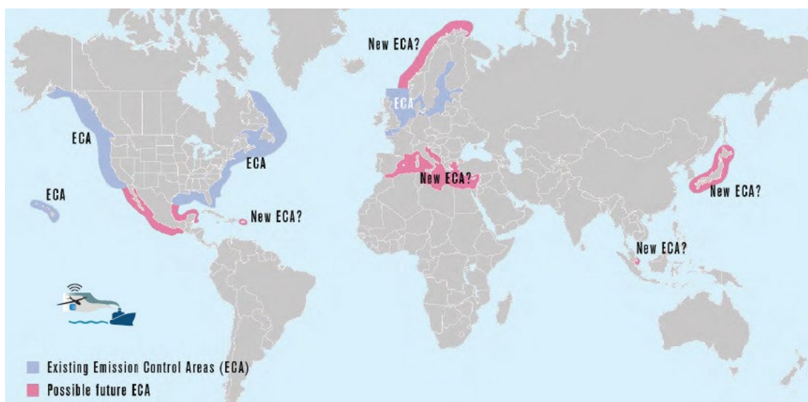
Figure 1-1 Emission control areas (adapted from CLS 2015)
