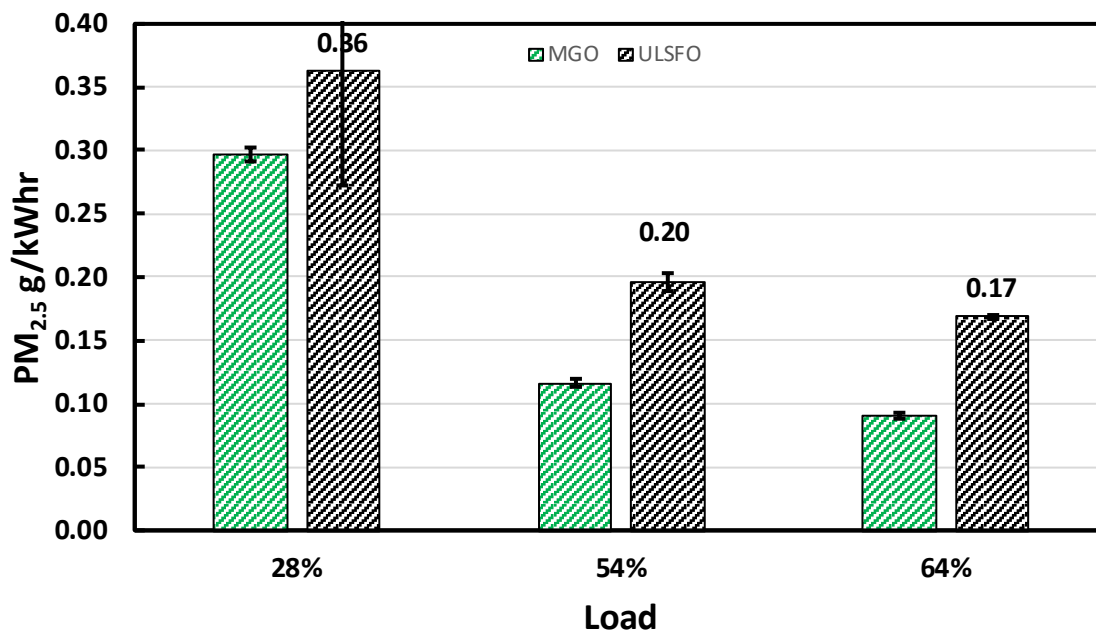
Figure 3-10 PM 2.5 Emissions for the AE in g/kWhr
