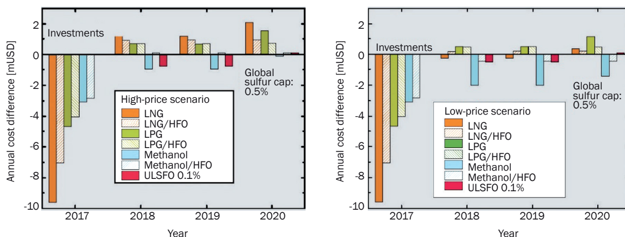
Figure 5 – Annual cost differences for the various fuel variants, based on two fuel price scenarios [12]
