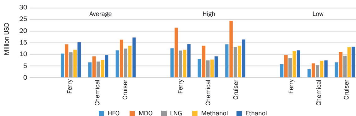
Figure 2 – Annual fuel costs for each ship type in million USD [8]
