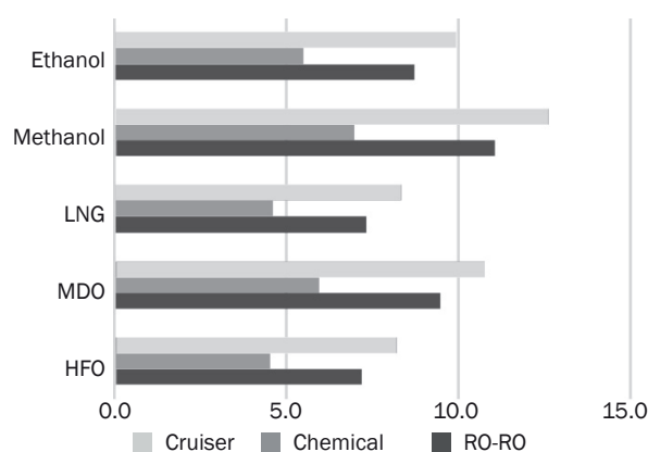
Figure 4 – Annual fuel cost for different fuel and ship types in million USD
