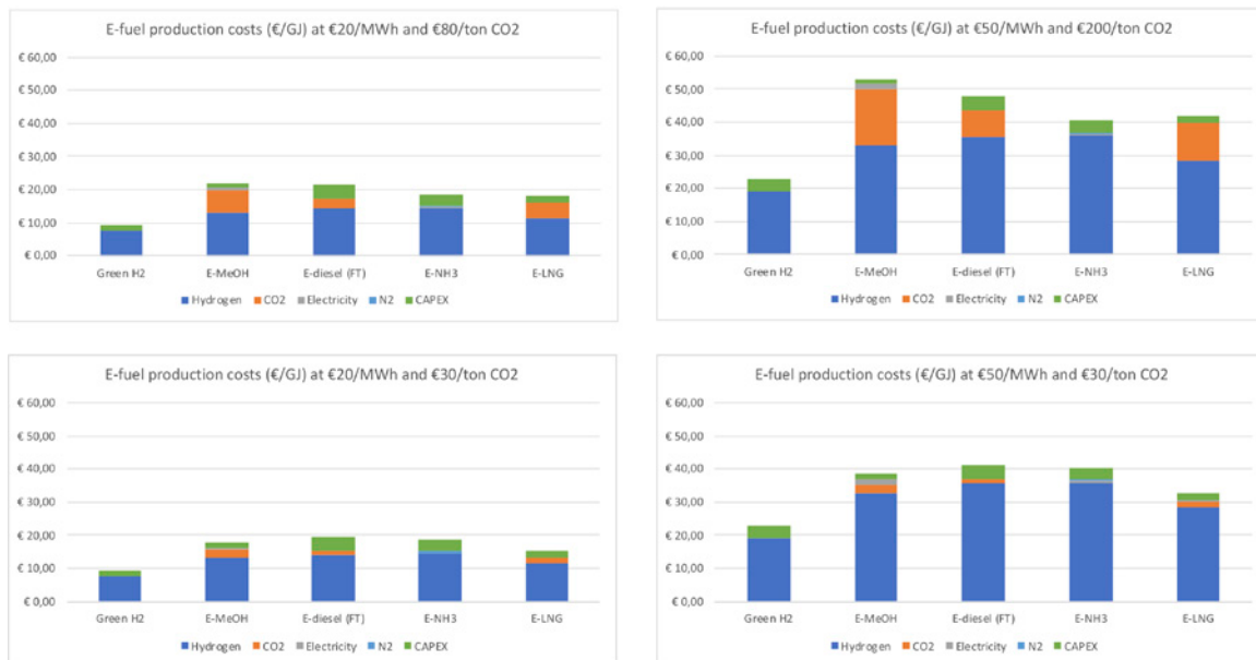
Figure 2 Production costs at different price levels for electricity and CO 2 . High CO 2 costs are associated with direct air capture and therefore dependent on electricity costs.
