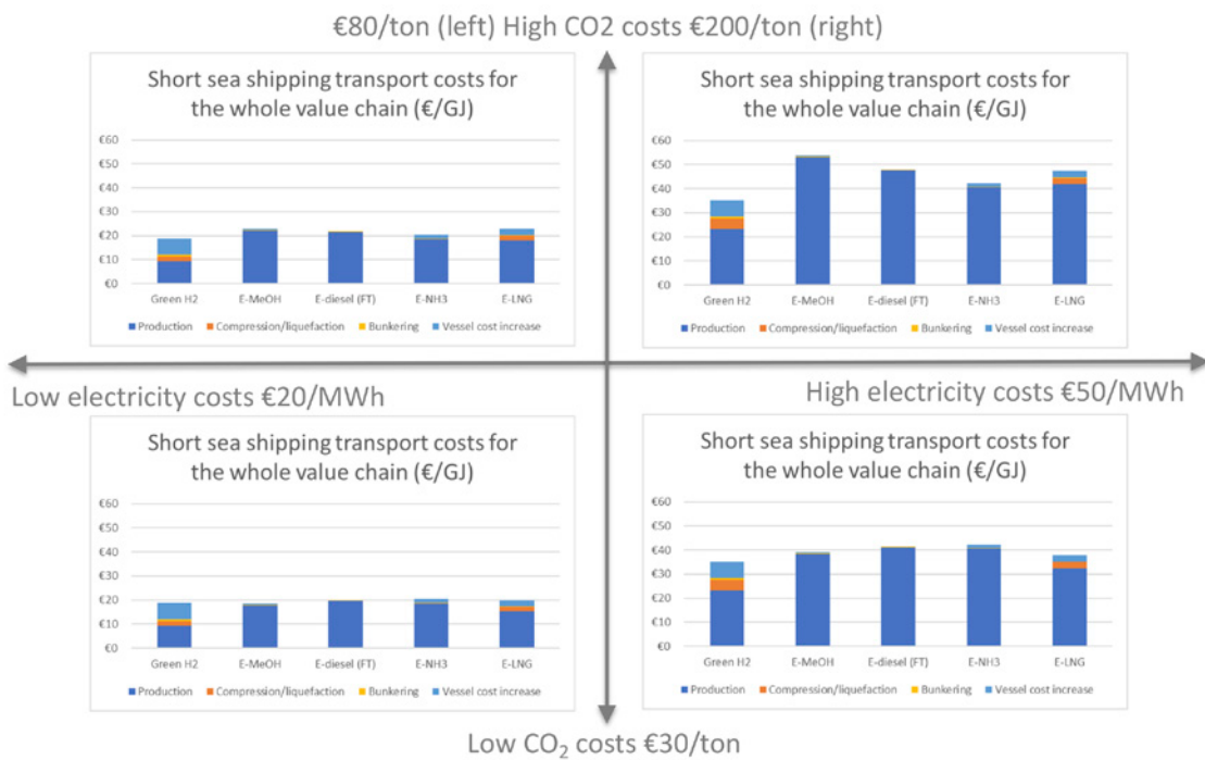
Figure 6. Value chain costs for short-sea shipping in four scenarios.
