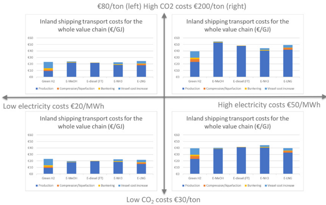
Figure 5. Value chain costs for inland shipping in four scenarios.
