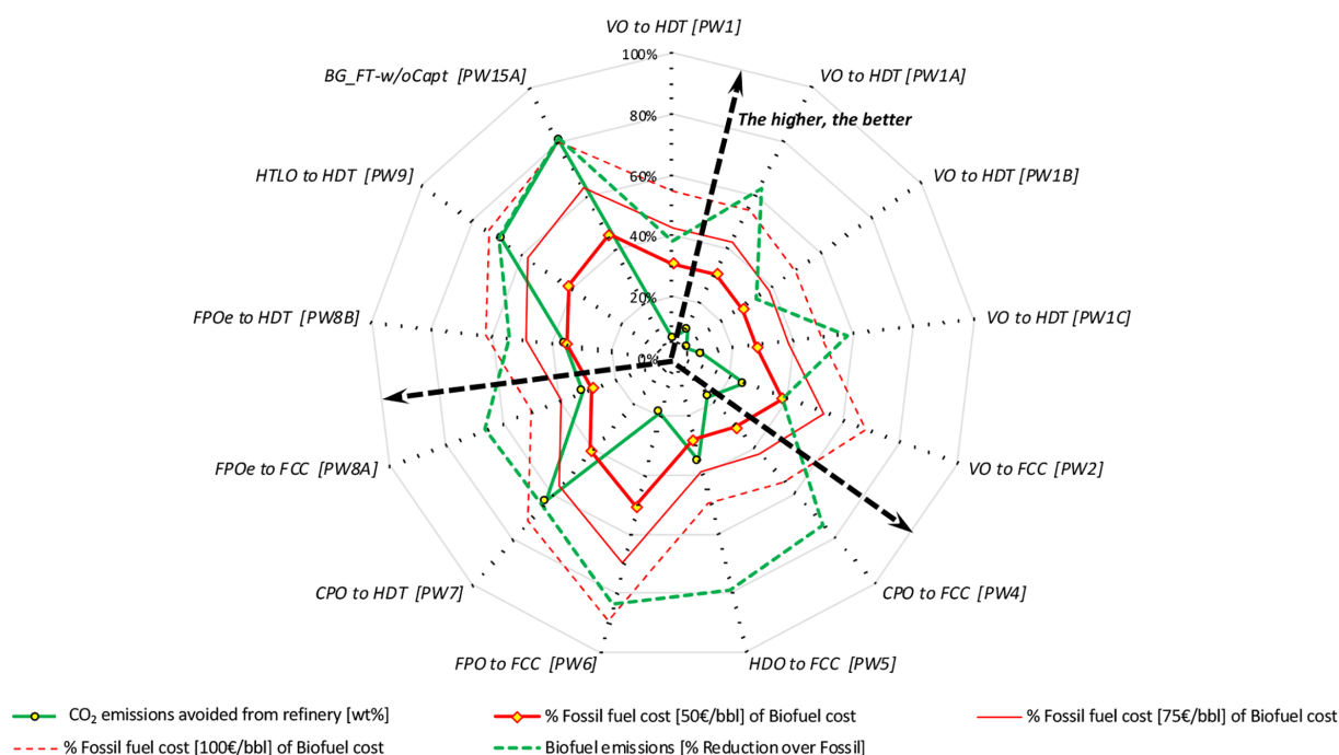
Figure 9. Percentage of CO 2 emissions avoided at the refinery and relative changes in biofuel emissions and production cost compared to fossil-fuel production. The higher the percentage of the category, the better is the CO-processing pathway compared to the fossil reference.
