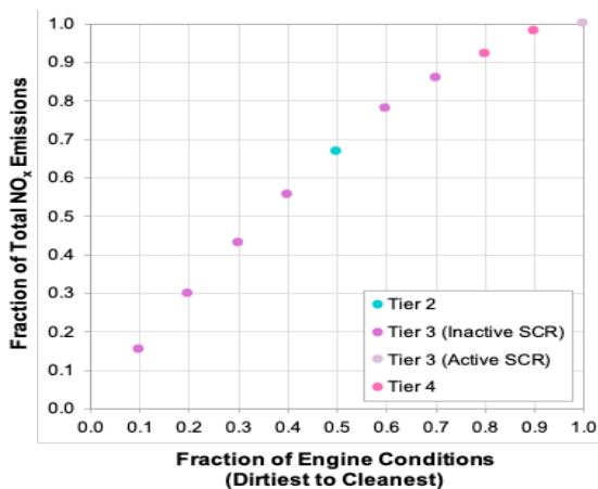
Figure 7. Cumulative Distribution of NOx Emissions
