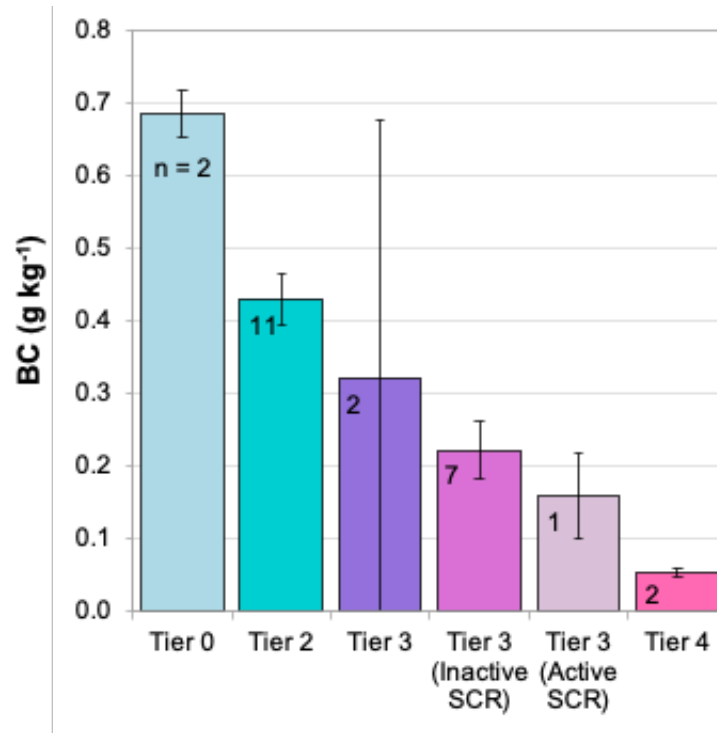
Figure 42: Average BC Emission Rates by Engine Tier
