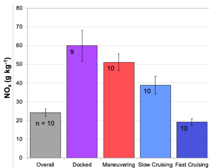
Figure 46: Fleet-Average NO x Emission Rates
