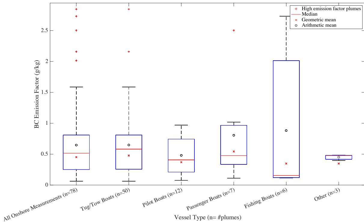
Figure 61: Onshore Emission Factor Distributions by Vessel Type
