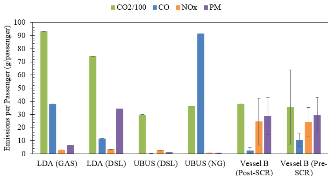
Figure 35: Comparison of Emissions per Passenger by Travel Mode (Vessel B)
