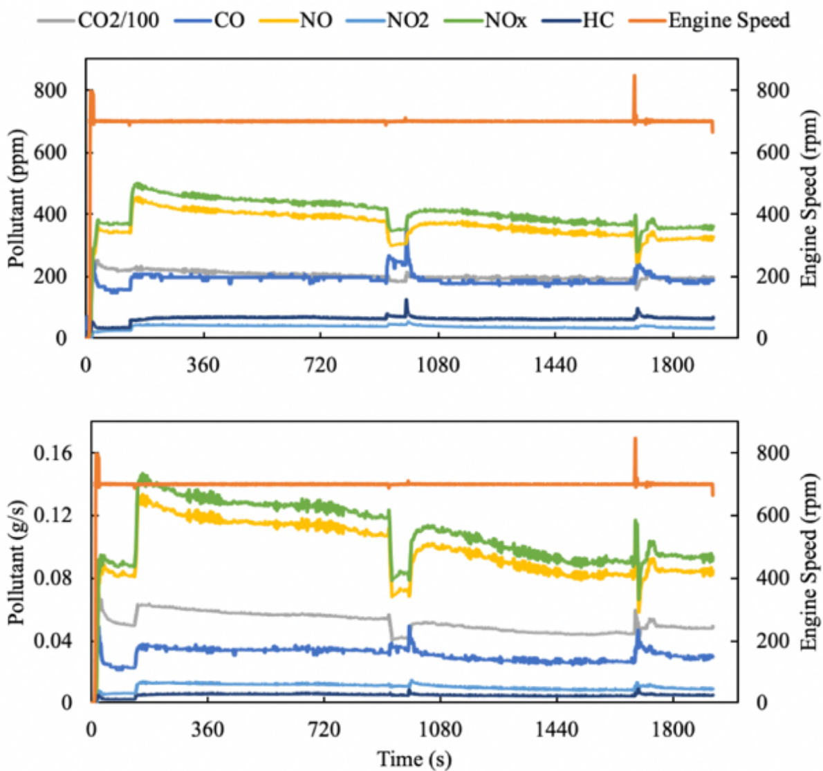
Figure 19: Vessel A Gaseous Cold Start Emissions and Engine Speed
