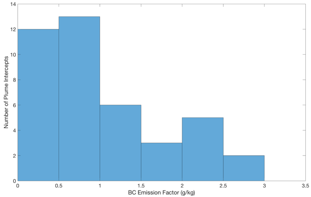
Figure 56: Dry Exhaust Fishing Boat Emission Factor Distribution
