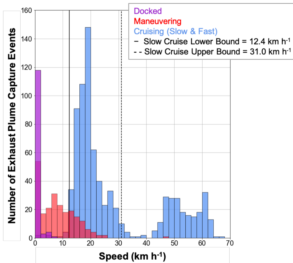
Figure 39: Speed Distributions by Operating Mode
