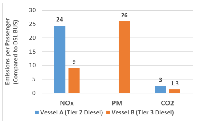
Figure 2. Emissions per Passenger (Diesel Vessel vs. Diesel Bus)
