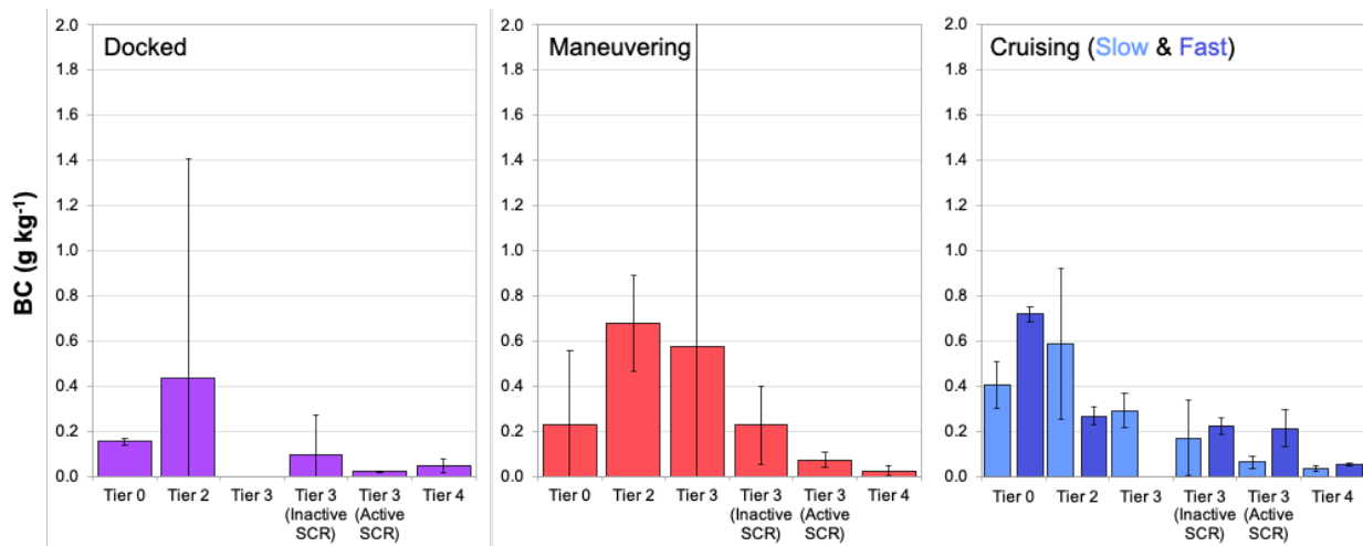
Figure 43: Average BC Emission Factors by Engine Tier and Operating Mode
