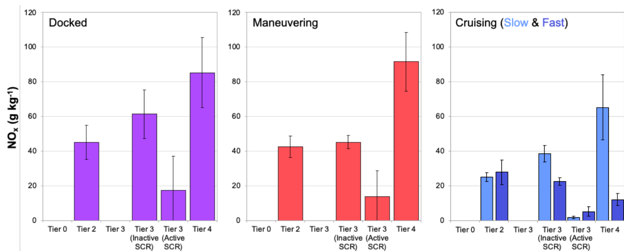
Figure 48: Average NO x Emission Factors by Engine Tier and Operating Mode
