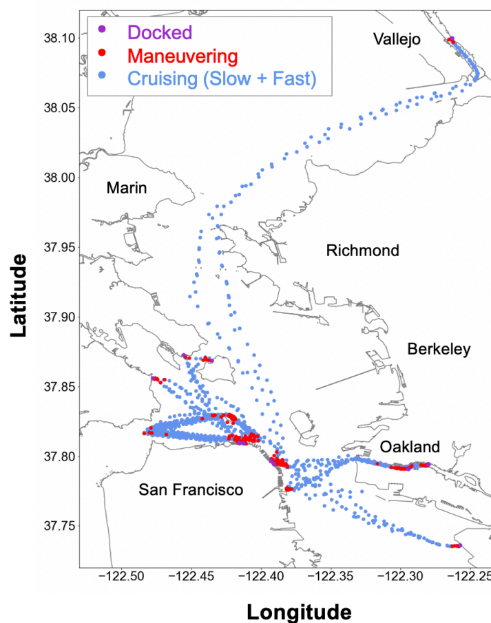
Figure 40: Map of All Measurements, Categorized by Operating Mode
