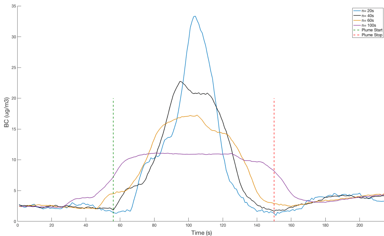
Figure 73: Effect of Different Moving Average Windows on BC Peaks
