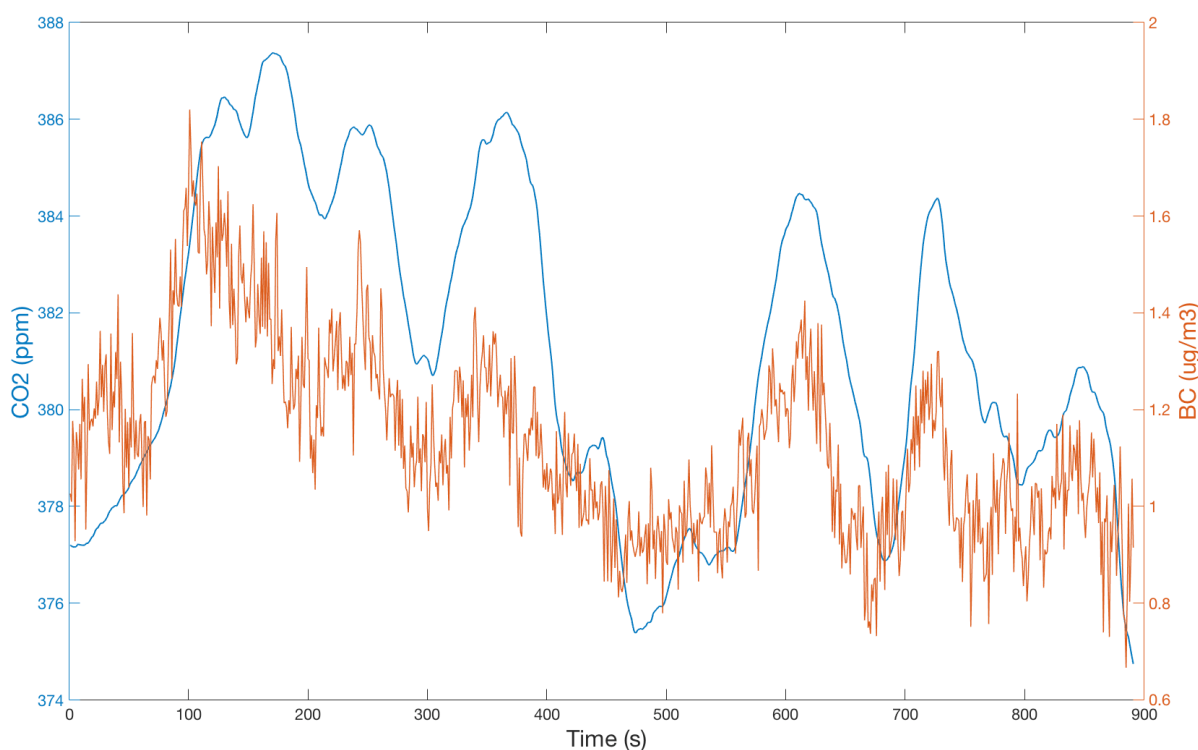
Figure 69: Example of Low Concentration BC Peak and Corresponding CO 2 Signal
