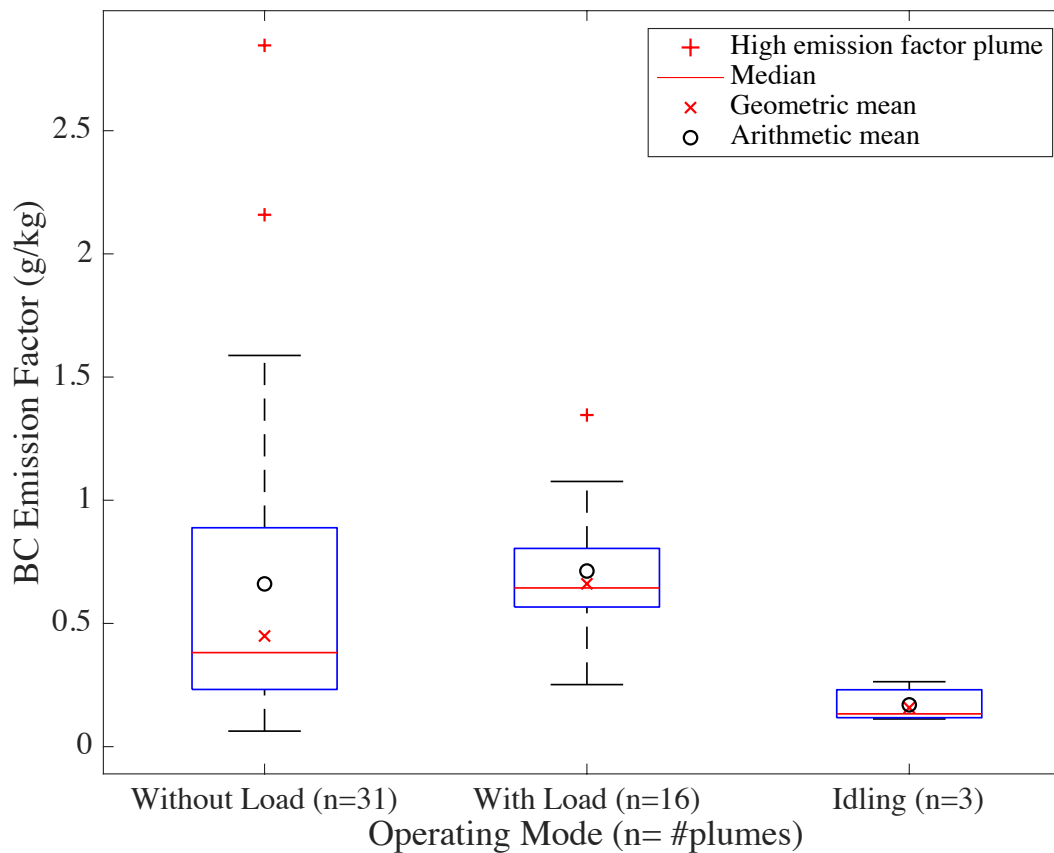
Figure 62: Tug/Tow Boat Emission Factor Distributions by Operating Mode
