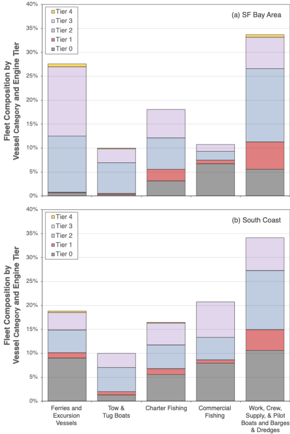
Figure 2: Composition of CHC Fleets by Engine Tier
