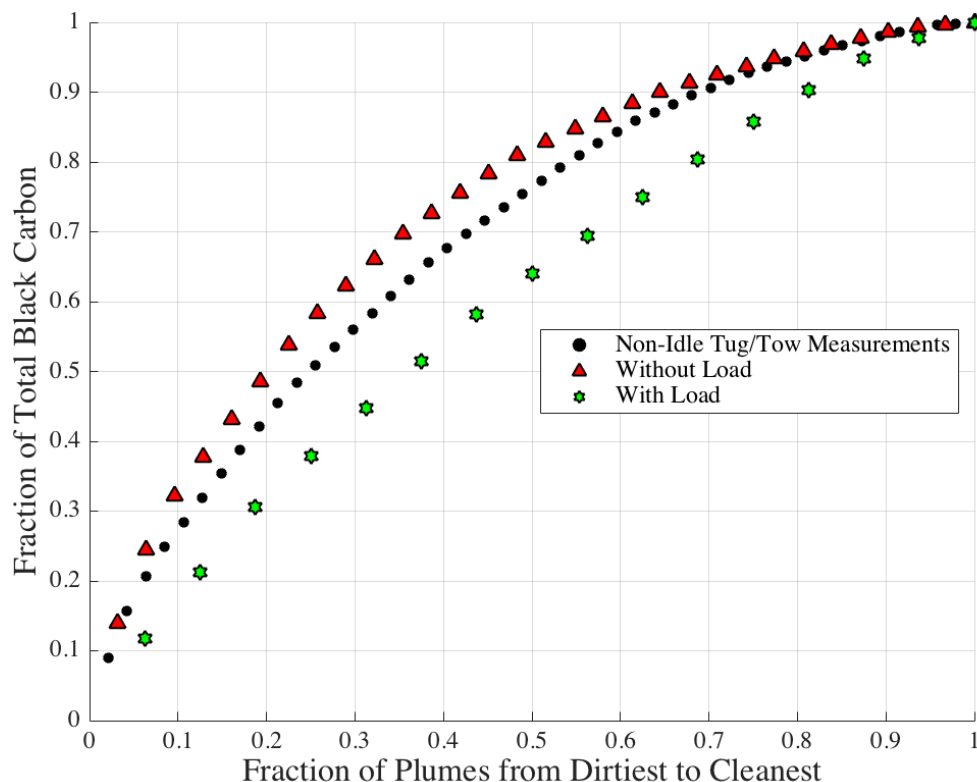
Figure 67: Cumulative Emissions Distributions for Tug/Tow Boats
