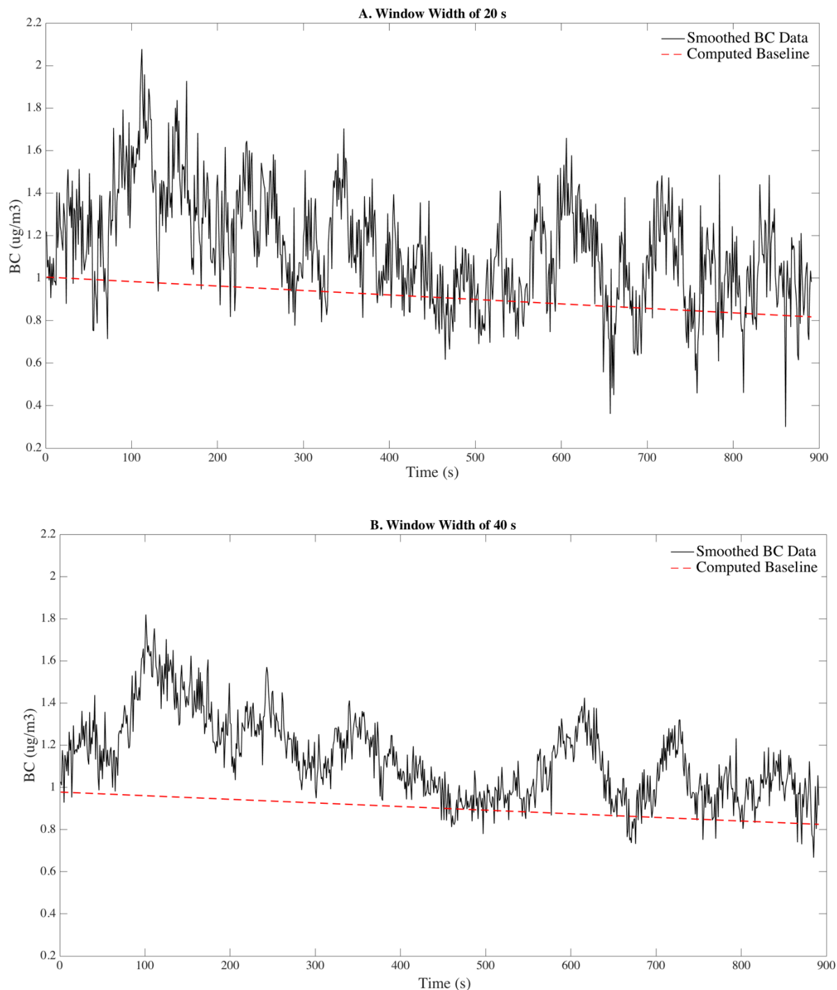
Figure 72: Example of Moving Baseline Calculated with Different Smoothing Windows
