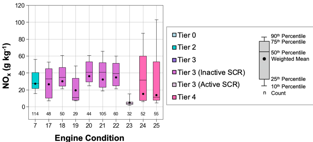
Figure 49: NO x Emission Factor Distributions for Each Measured Engine Condition
