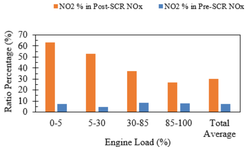
Figure 29: NO 2 Percentage in NO x for Vessel B
