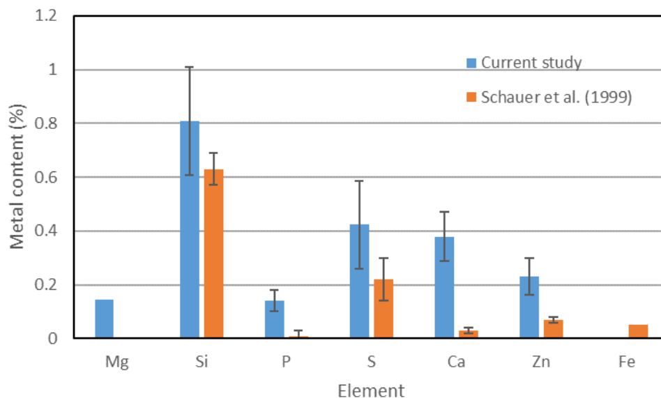
Figure 32: XRF Analysis of PM Samples from Vessel B, Pre-SCR
