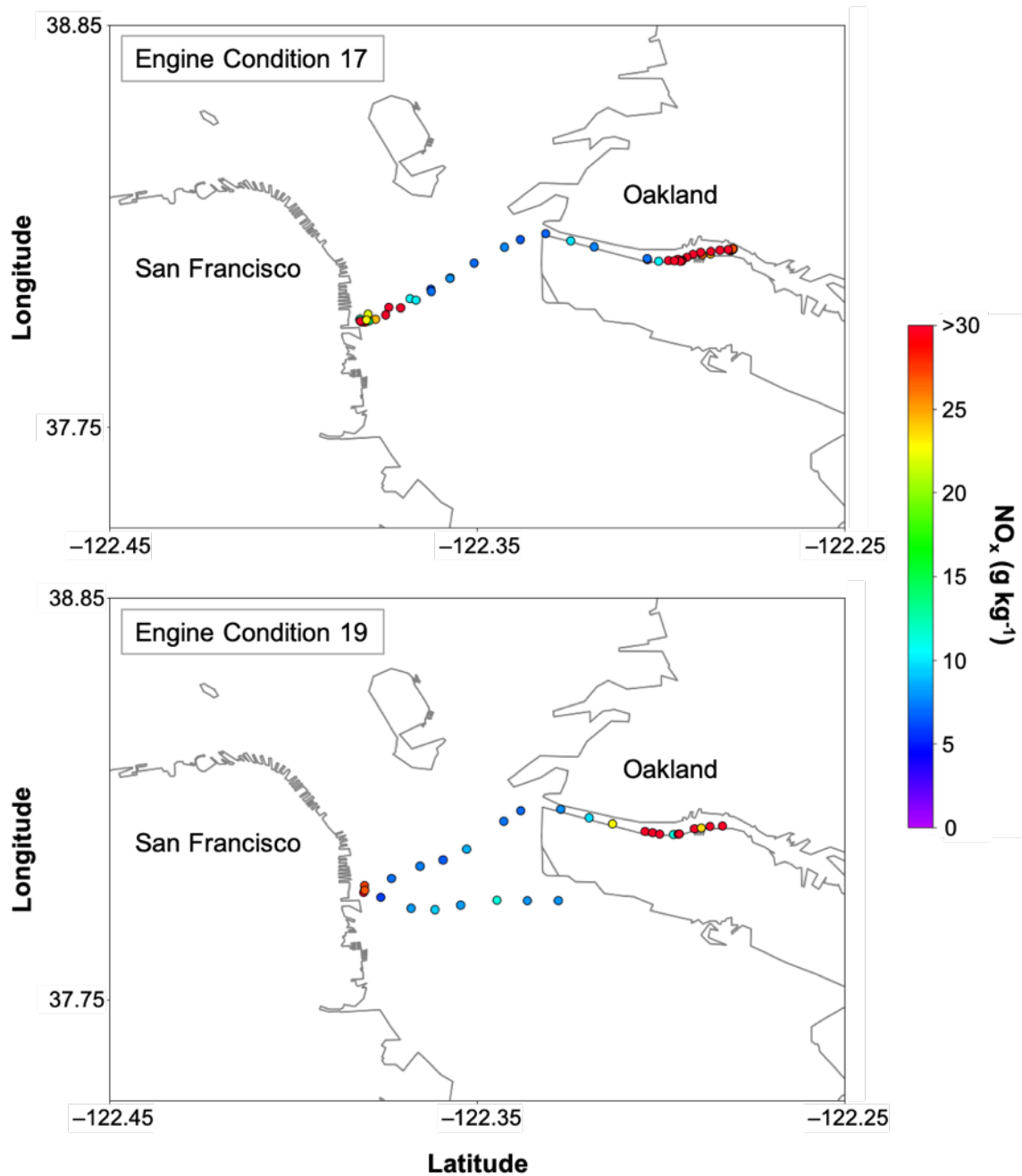
Figure 52: Example of Operating Mode-Dependence of SCR Activity
