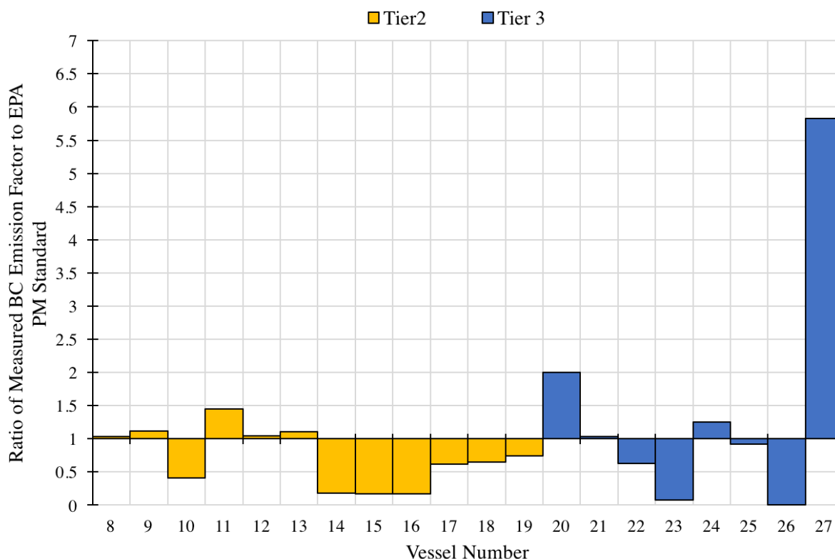
Figure 65: Ratio of Measured BC Emission Factors to EPA PM Standards
