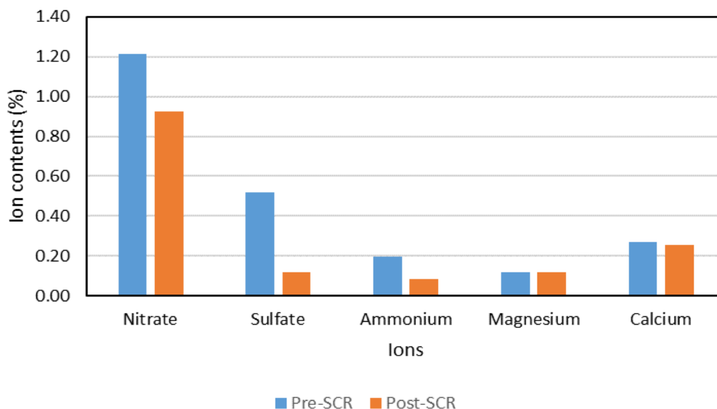
Figure 33: IC Analysis for PM Samples from Vessel B, Pre- and Post-SCR
