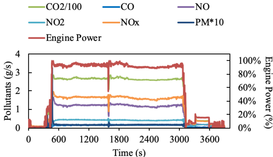
Figure 30: Example Time Series of Emissions for Vessel B, Post-SCR
