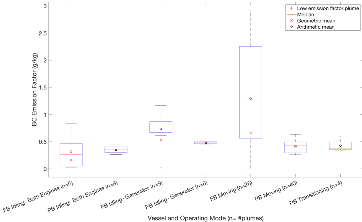
Figure 58: Emission Factor Distributions by Vessel and Operating Mode
