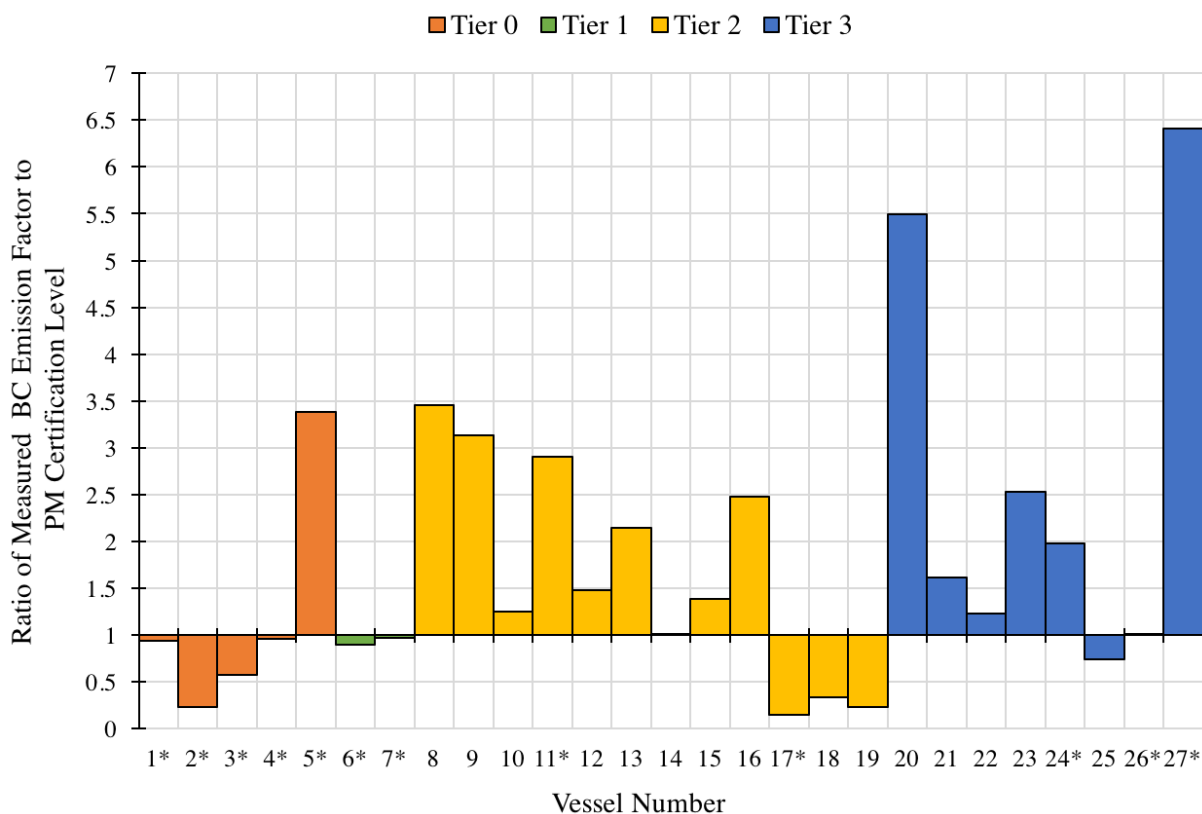
Figure 64: Ratio of Measured BC Emissions Factors to PM Certification Levels
