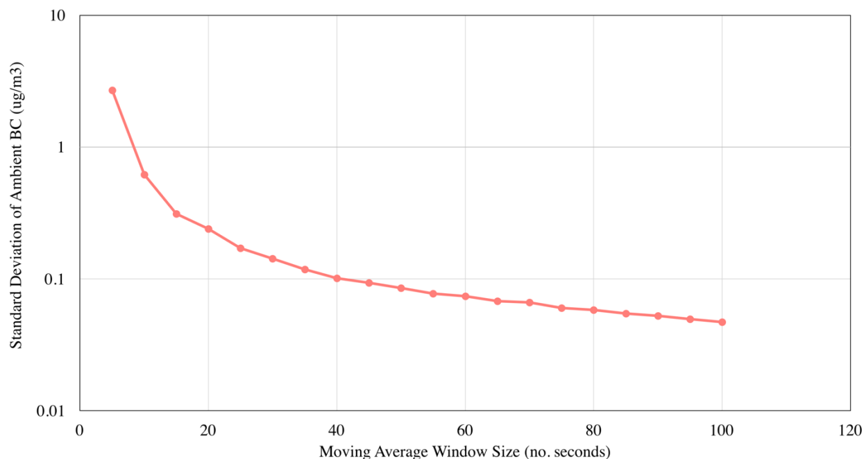
Figure 71: Noise in ABCD Measurements as a Function of Moving Average Window Size
