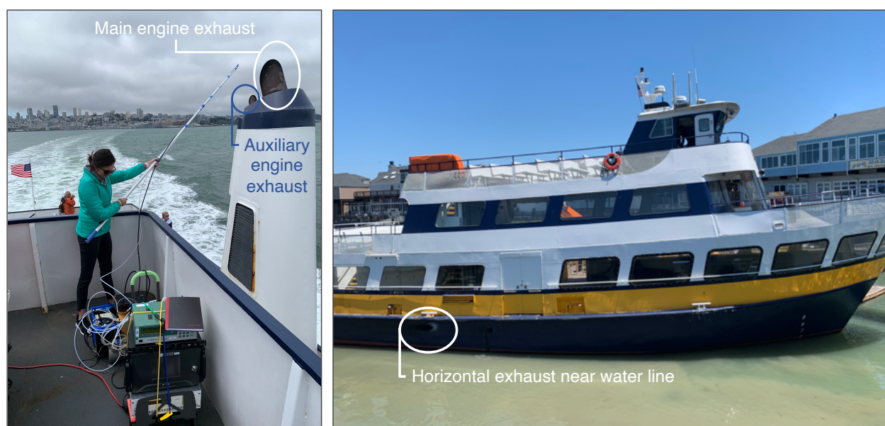
Figure 36: Exhaust Configurations and Plume Capture Sampling Method
