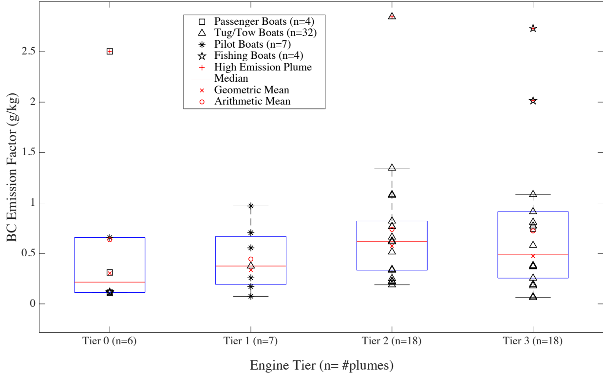
Figure 63: Onshore Measurement Distributions by Engine Tier
