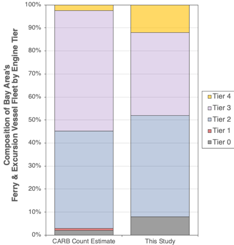
Figure 38: Composition of Bay Area Ferry and Excursion Vessel Fleet by Engine Tier
