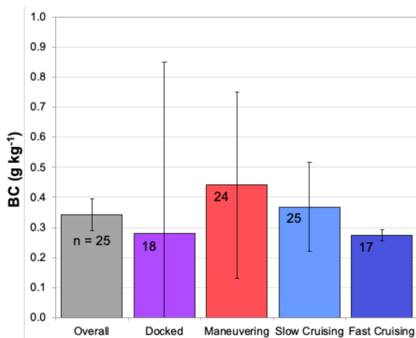
Figure 41: Fleet-Average BC Emission Rates by Operating Mode
