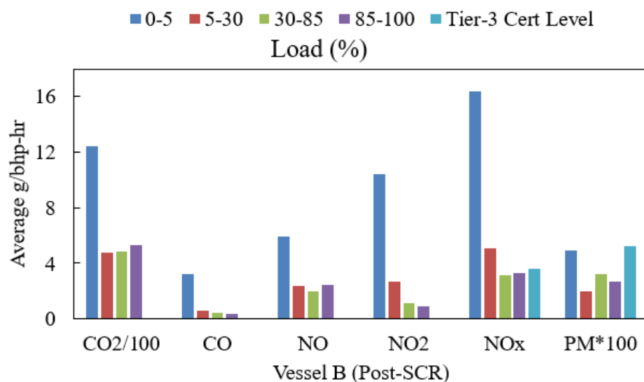
Figure 27: Average Emissions by Engine Load for Vessel B, Post-SCR
