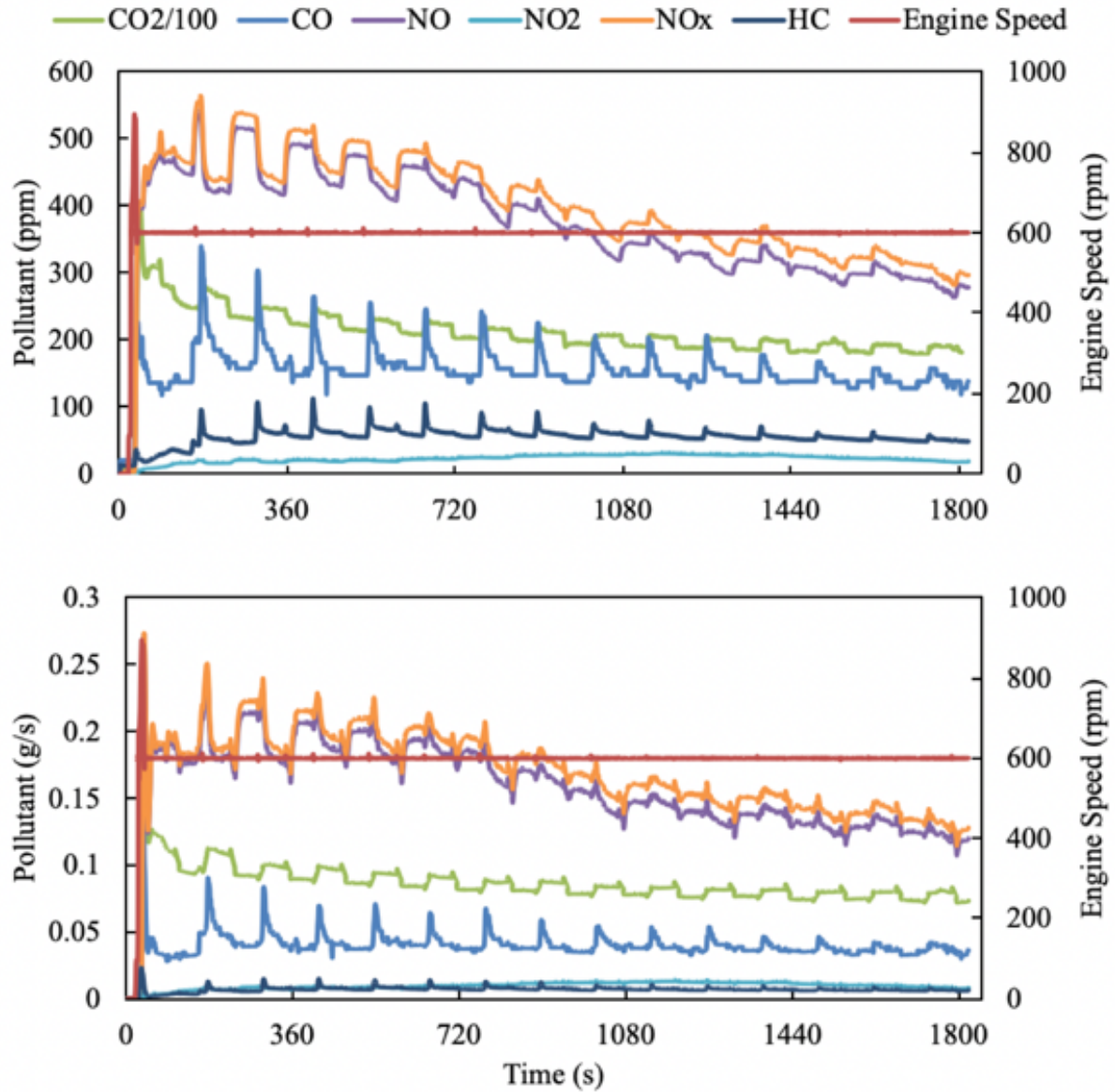
Figure 20: Vessel B Gaseous Cold Start Emissions and Engine Speed
