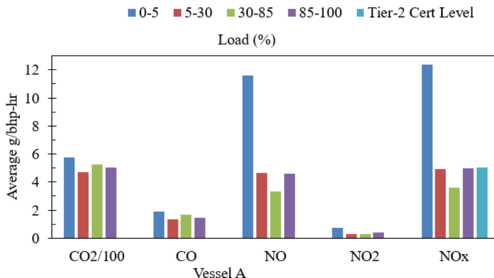
Figure 23: Average Emissions by Engine Load for Vessel A
