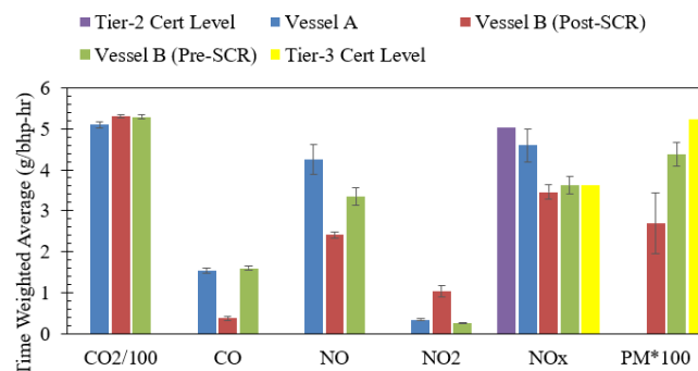
Figure 1. Average Emission Rates for Both Vessels
