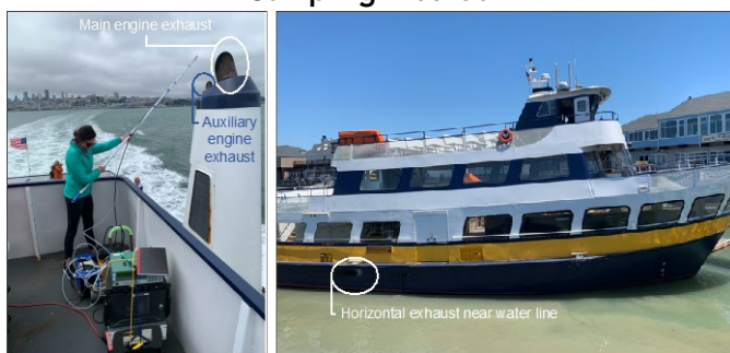
Figure 3. Exhaust Configurations and Plume Capture Sampling Method
