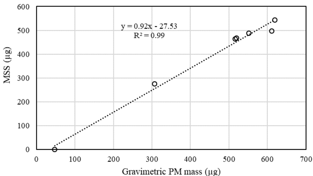
Figure 31: Comparison of PM Mass Measurement Methods
