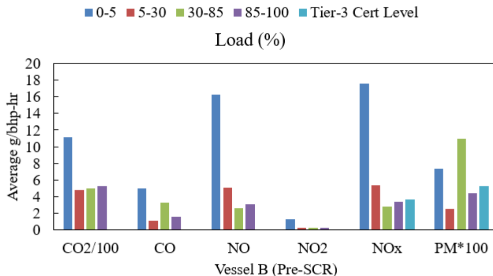
Figure 25: Average Emissions by Engine Load for Vessel B, Pre-SCR
