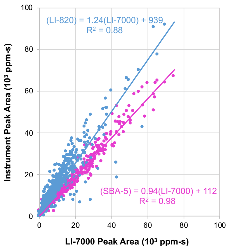
Figure 37: CO_2 Peak Areas Calculated with the LI-820 and SBA-5 vs the LI-7000
