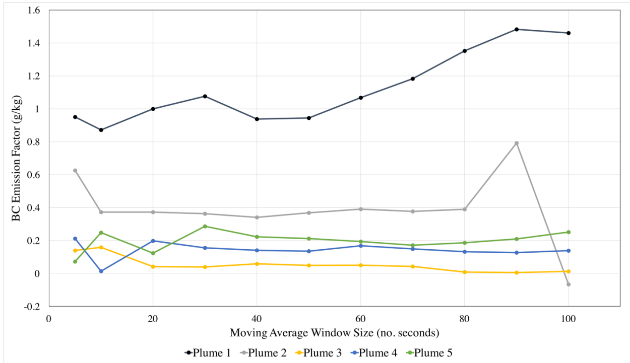
Figure 70: Impact of Different Moving Average Windows on Calculated Emission Factors
