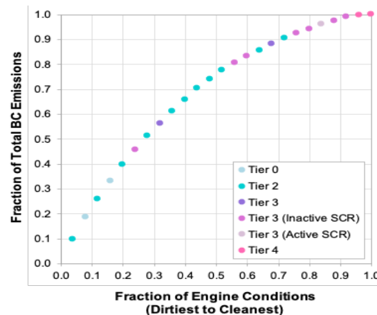
Figure 5. Cumulative Distribution of BC Emissions
