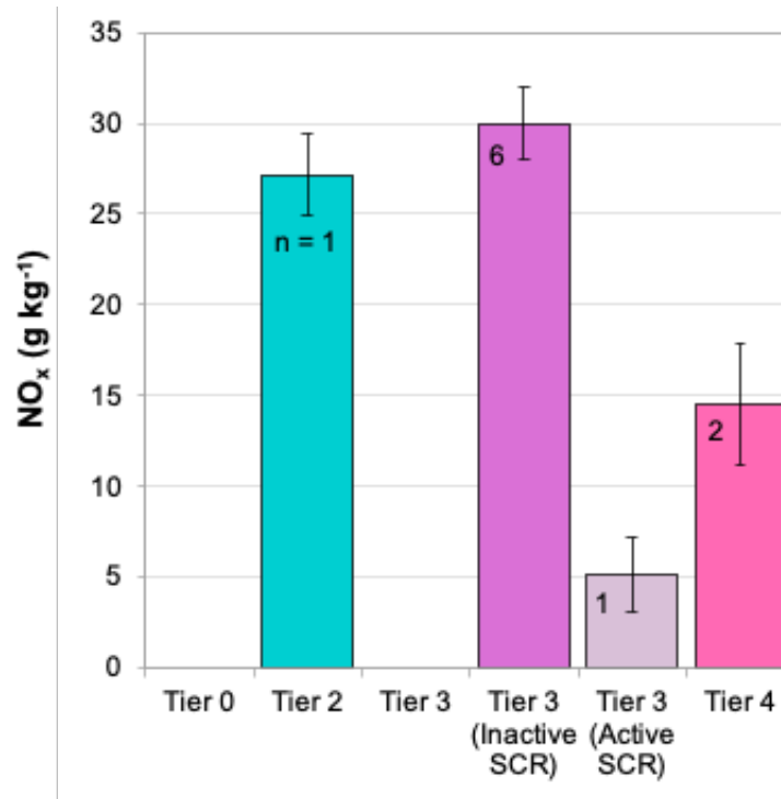
Figure 47: Average NO x Emission Rates by Engine Tier
