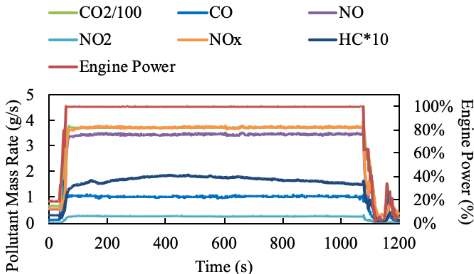
Figure 24: Example Time Series of Emissions for Vessel A
