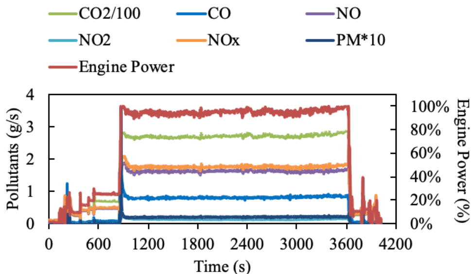
Figure 26: Example Time Series of Emissions for Vessel B, Pre-SCR
