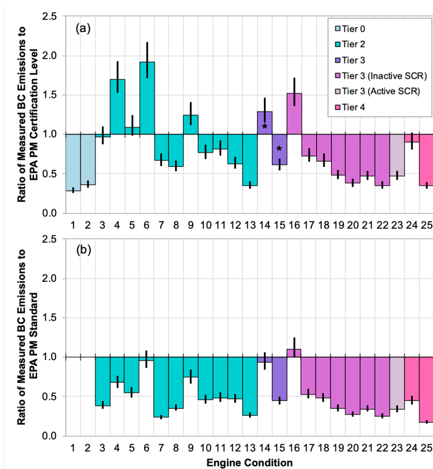
Figure 54: Ratio of Measured BC and EPA Values
