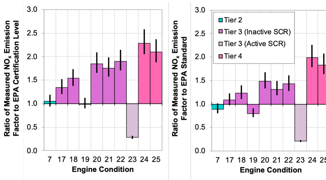
Figure 55: Ratio of Measured NO x and EPA Values
