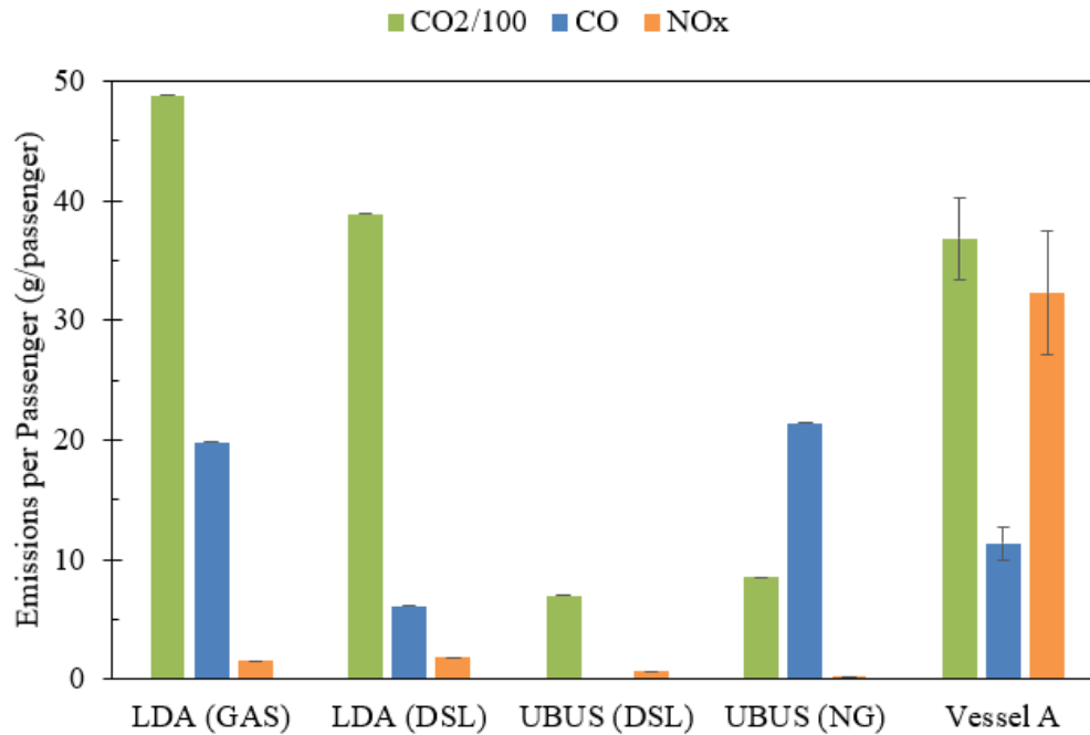
Figure 34: Comparison of Emissions per Passenger by Travel Mode (Vessel A)
