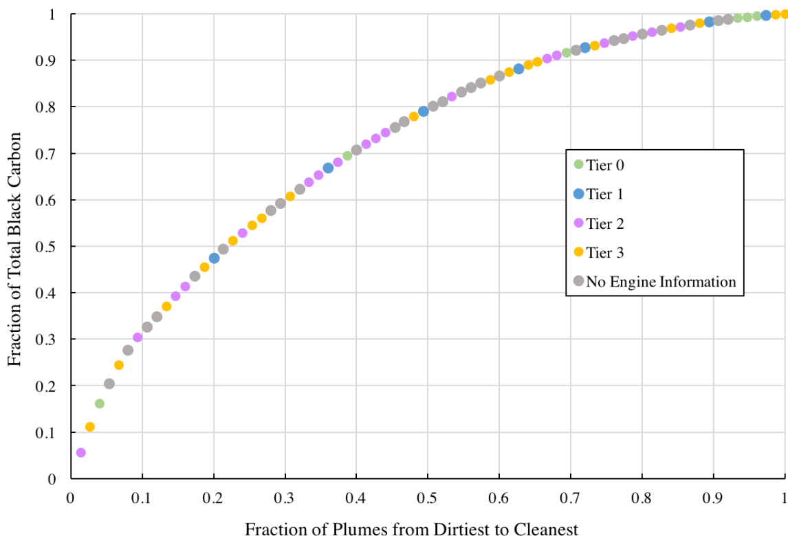
Figure 68: Cumulative Emissions Distribution by Engine Tier
