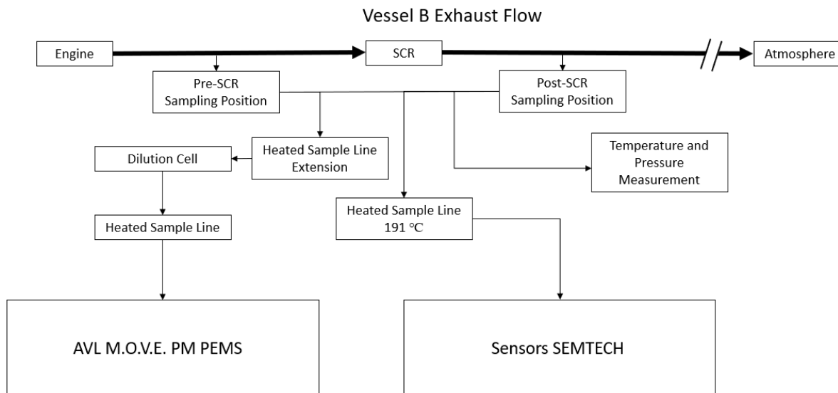
Figure 8: Exhaust Flow and Sampling Diagram for Vessel B
