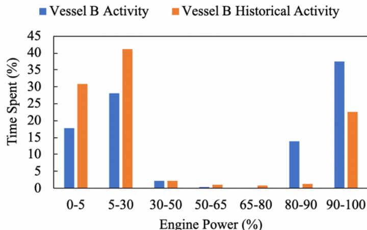
Figure 18: Historic Load and Testing Activity for Vessel B's Port Engine
