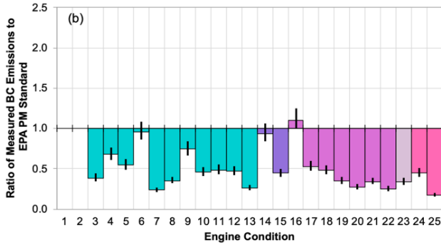
Figure 6. Ratio of Measured BC and EPA Values
