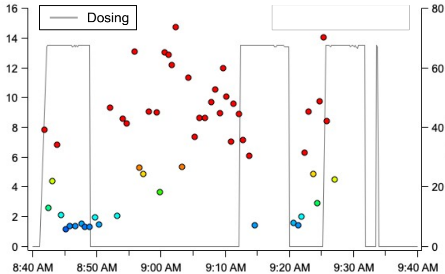
Figure 53: SCR Dosing Rate and Corresponding NO x Emission Factors
