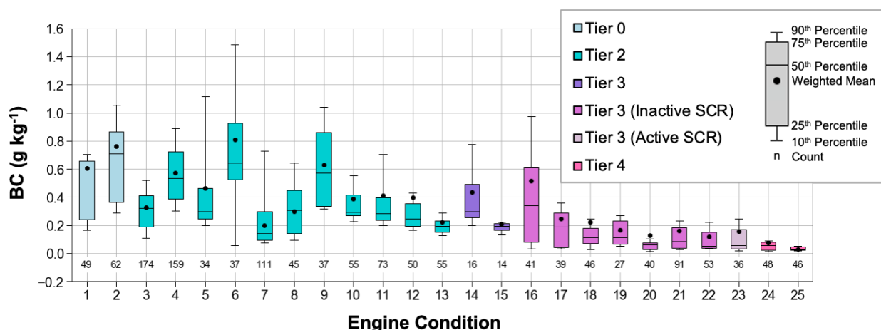
Figure 44: BC Emission Factor Distributions for Each Measured Engine Condition
