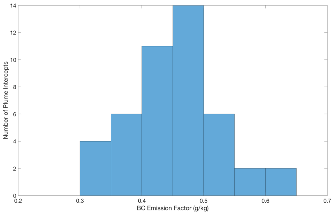
Figure 57: Wet Exhaust Passenger Boat Emission Factor Distribution
