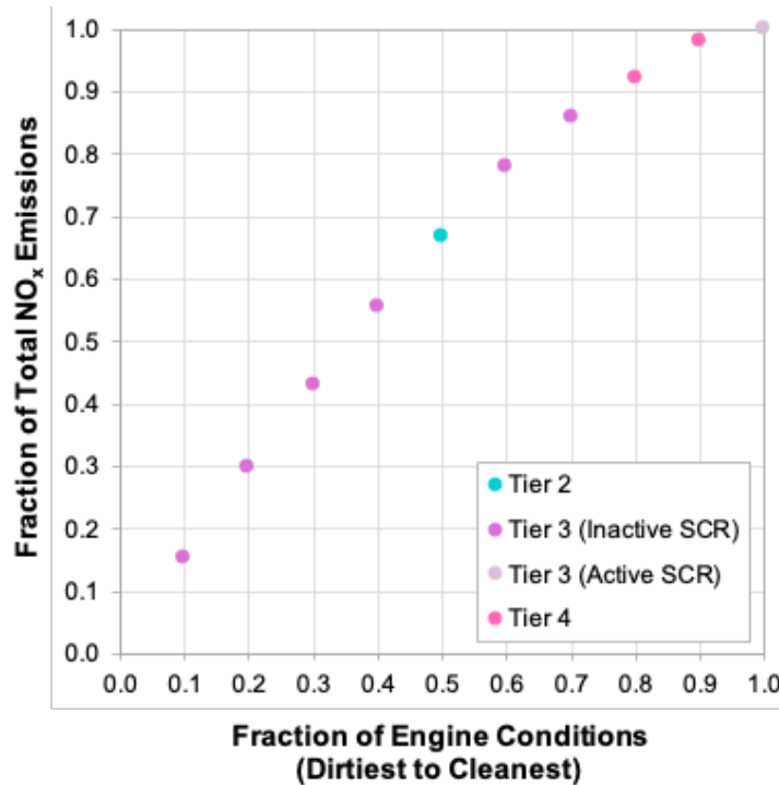
Figure 50: Cumulative Distribution of NO x Emissions
