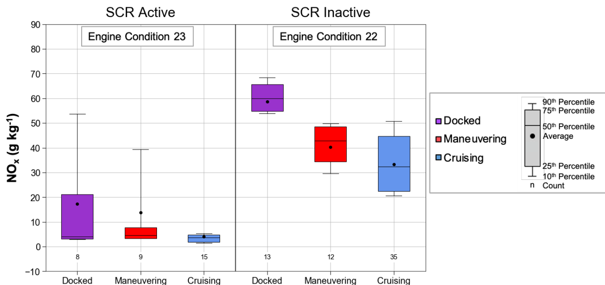
Figure 51: Case Study of SCR Effectiveness with Engine 19 Experiment
