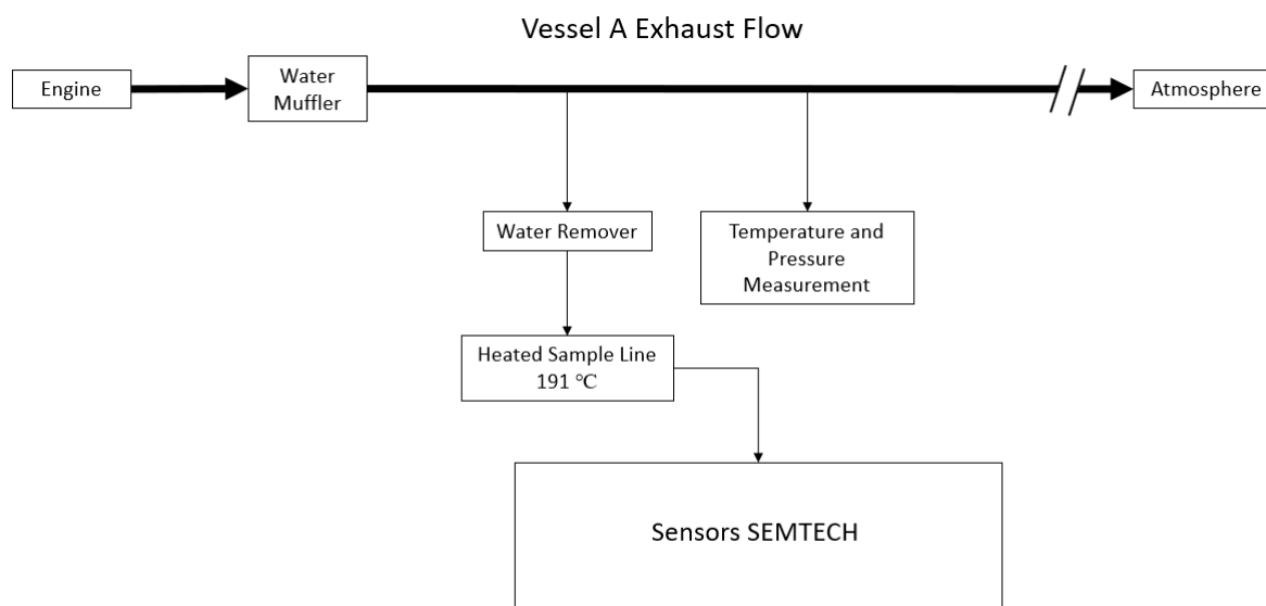
Figure 7: Exhaust Flow and Sampling Diagram for Vessel A
