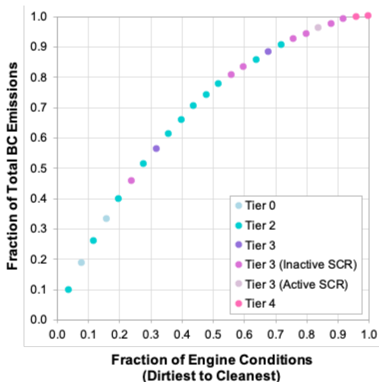
Figure 45: Cumulative Distribution of BC Emissions
