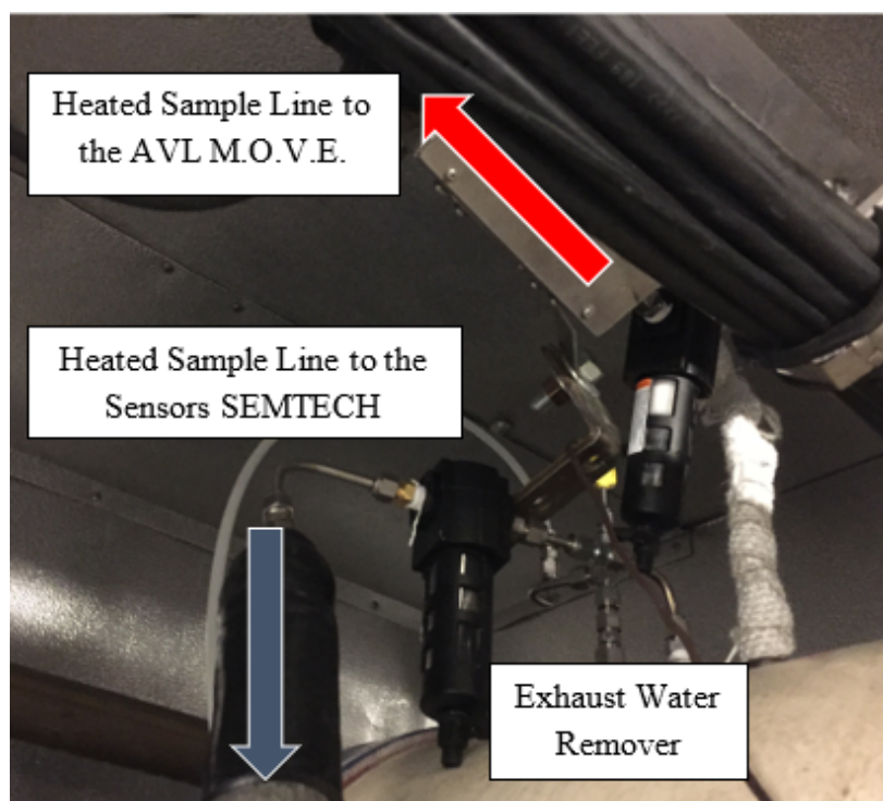
Figure 11: Exhaust Ports on Vessel A
