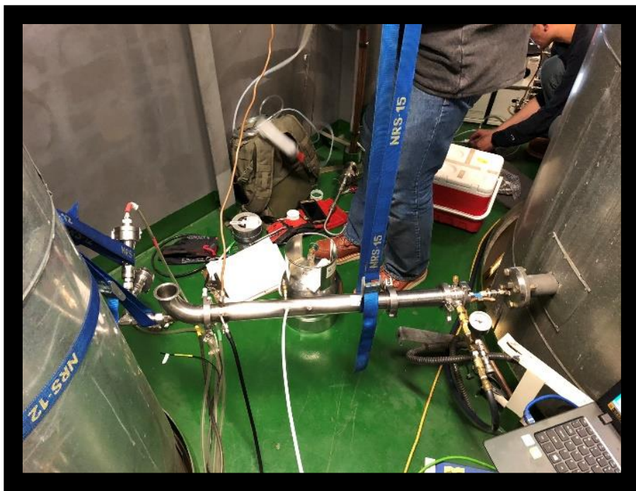
Figure C-2 Installation showing removal of cyclone.
