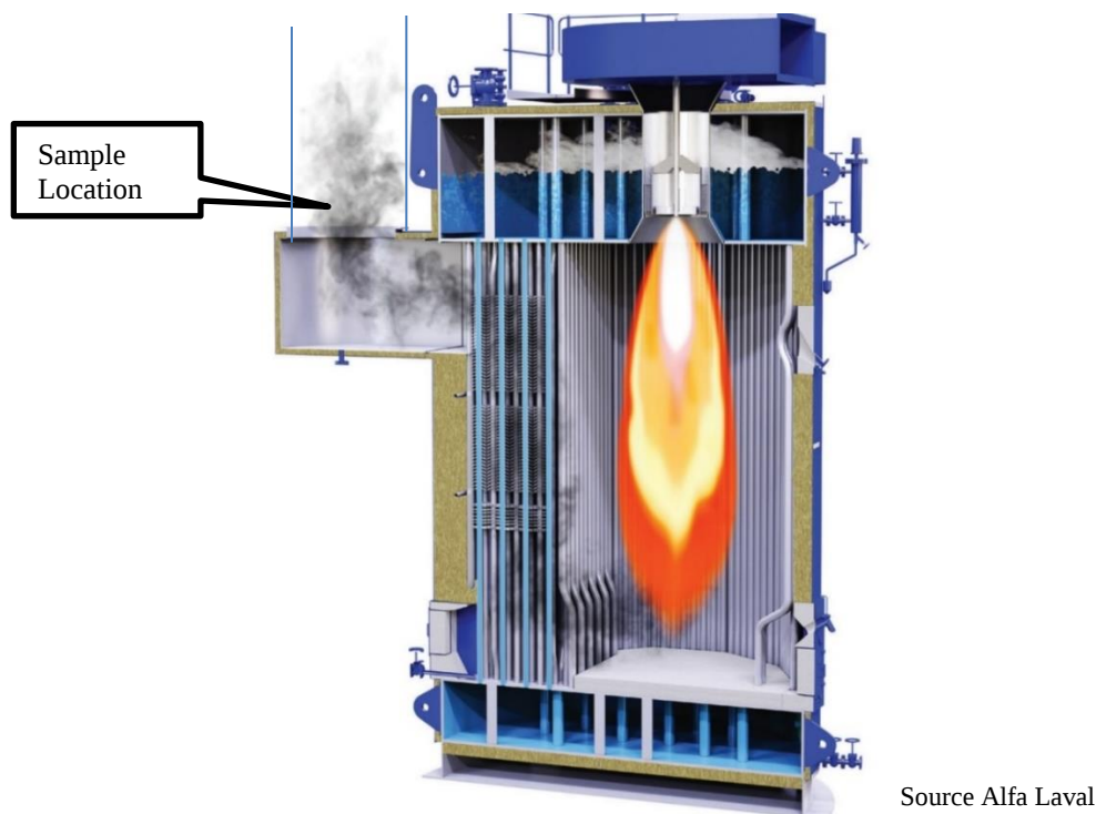
Figure 2-1 Design diagram of large frame boiler series
