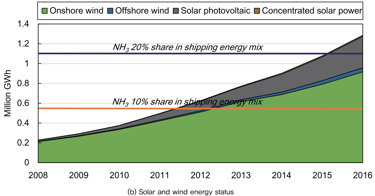
[Figure 7] Power Generation from Renewable Energy [17]
