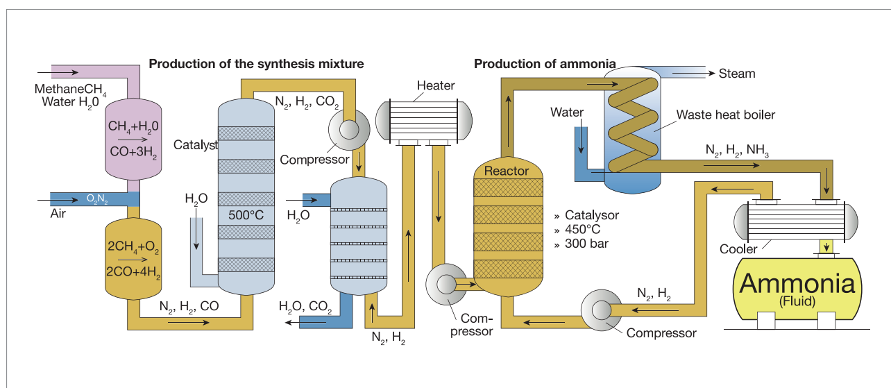
[Figure 5] Schematic Diagram of the Haber-Bosch Process
