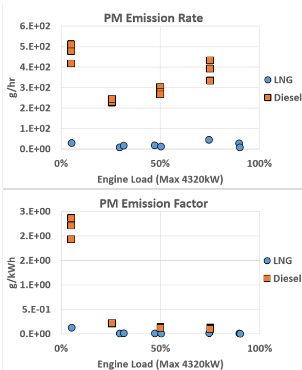
FIGURE 12 MODAL RATES AND FACTORS FOR PM MASS FOR LNG & DIESEL
