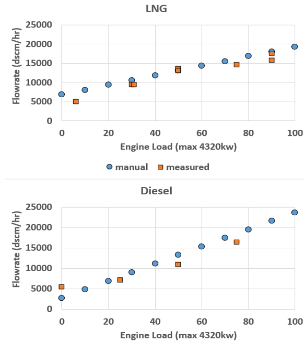
FIGURE 6 FLOW EXHAUST RATE IN DRY STANDARD CUBIC METER PER HOUR
