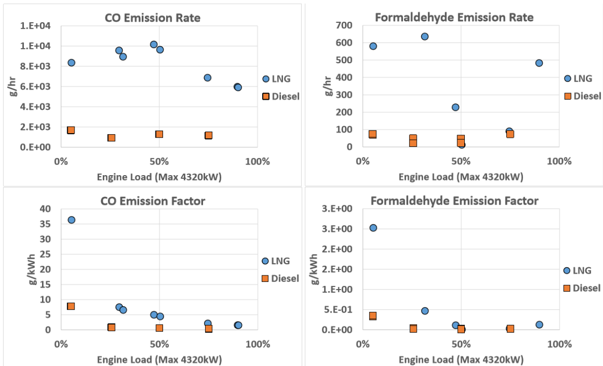
FIGURE 9 MODAL EMISSION RATES & FACTORS FOR CO & HCHO
