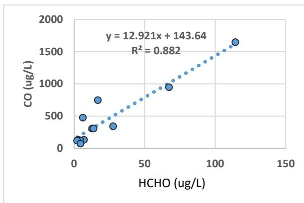
FIGURE 10 CORRELATION OF CO & HCHO
