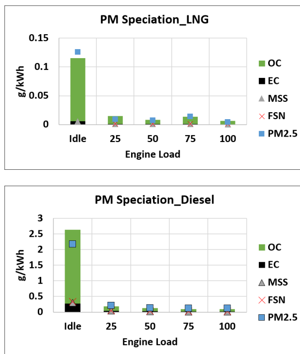
FIGURE 13 MODAL RATES AND FACTORS FOR PM FRACTIONS FOR LNG & DIESEL
