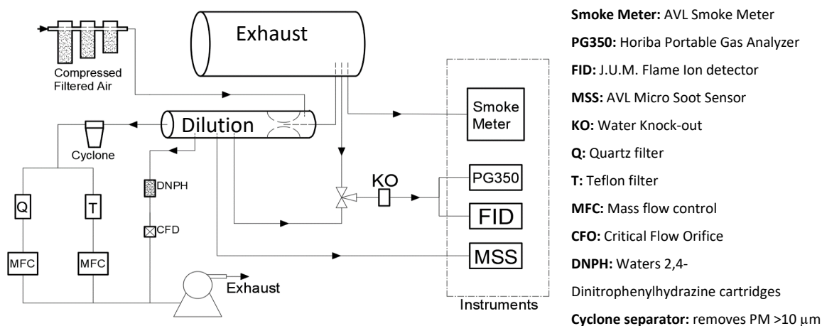
FIGURE 5 SCHEMATIC SHOWING LAYOUT OF UCR EQUIPMENT
