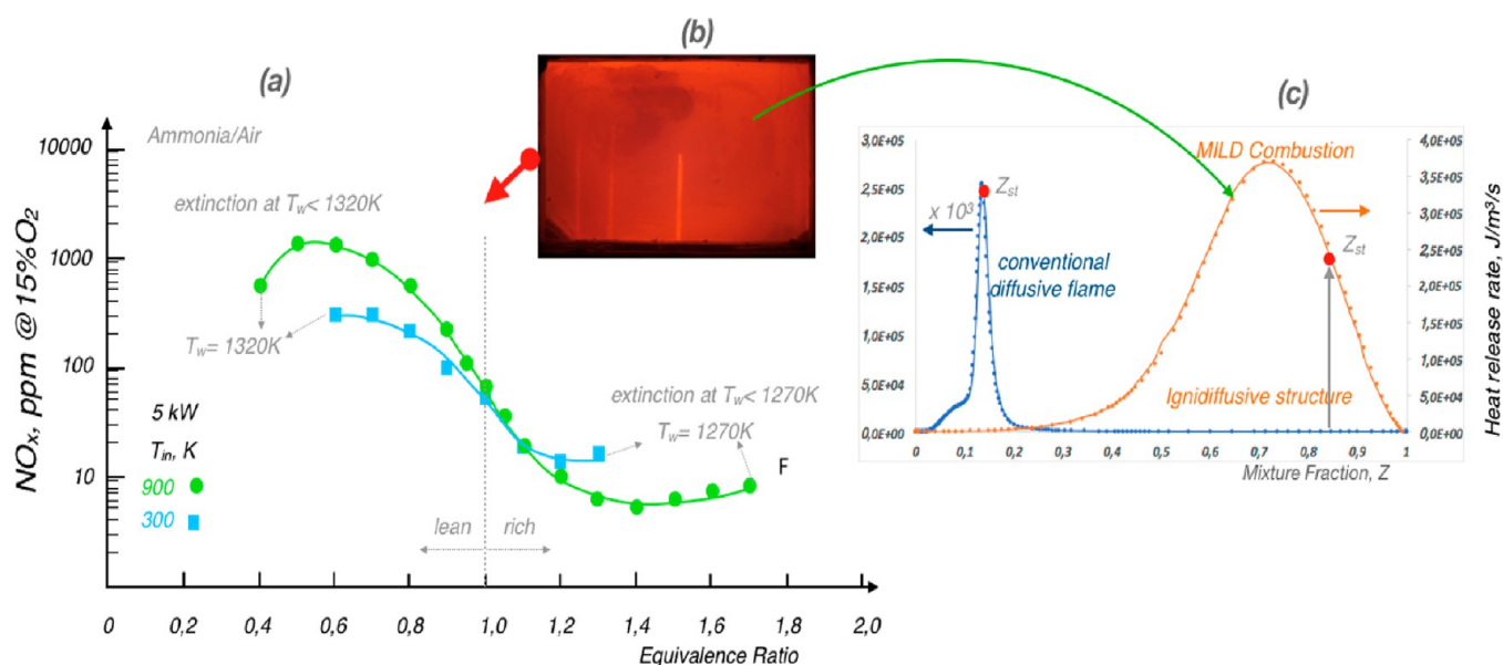
Figure 27. Ammonia MILD combustion: (a) NO x emission, (b) example of no visible flame, and (c) example of an igni-diffusive structure.
