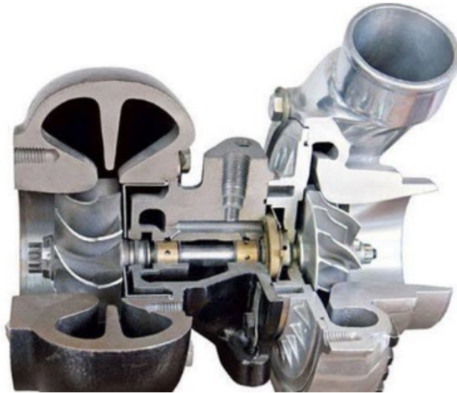
Figure E-5b. Waste-Gated Turbocharger Cutaway 31
