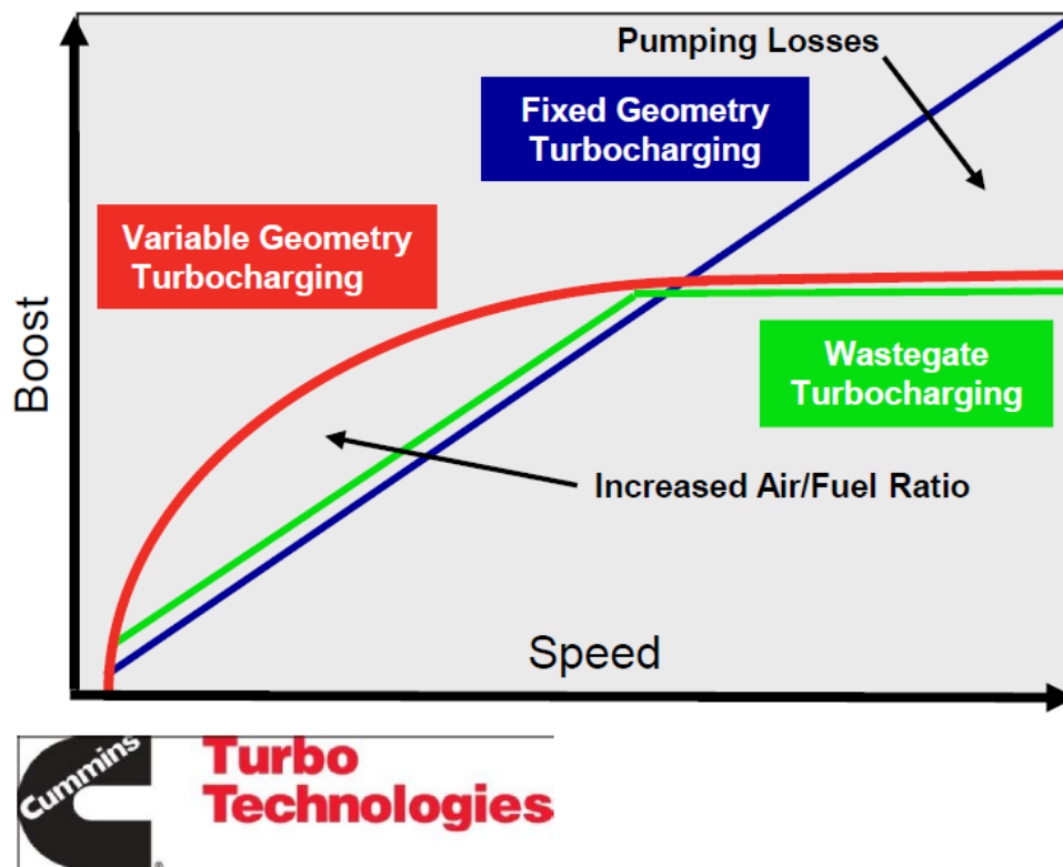
Figure E-6. Cummins Turbocharger Performance: Boost Versus Turbine Speed in Fixed Geometry, Wastegated, and Variable Geometry Turbocharging (VGT) 34
