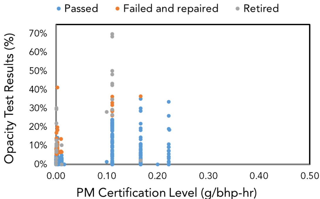
Figure E-25. RTG Opacity Test Results and PM Certification Level
