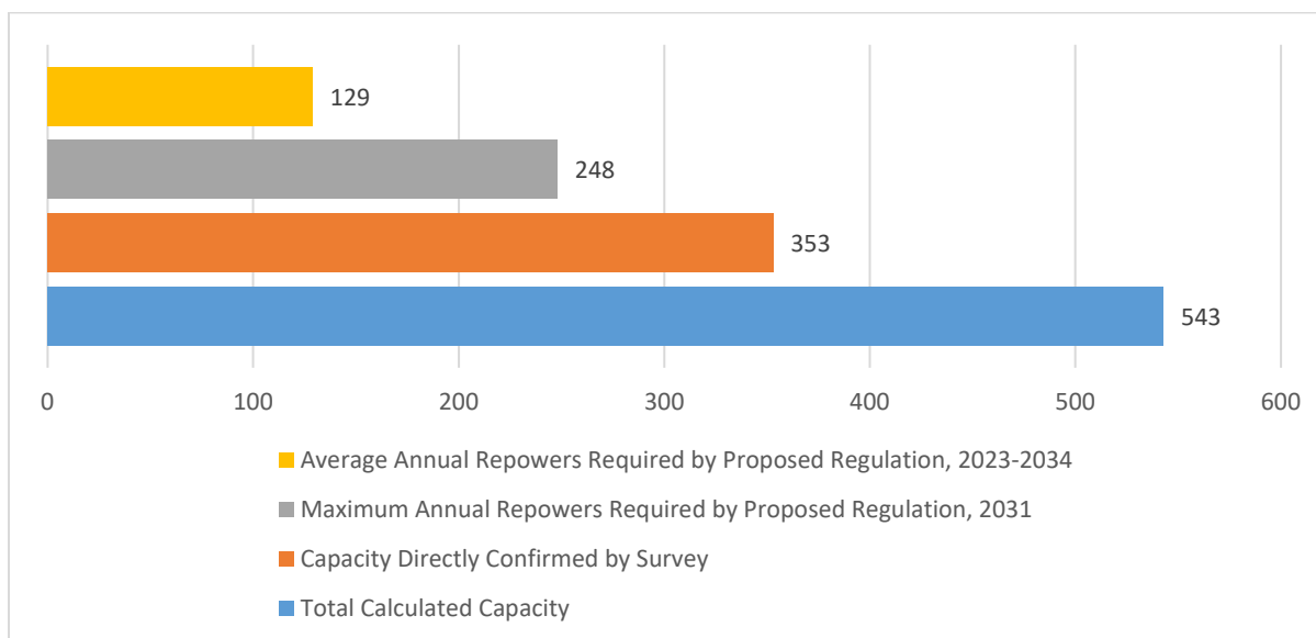
Figure E-13. Comparison of Repower Capacity and Number of Repowers Required by the Proposed Amendments
