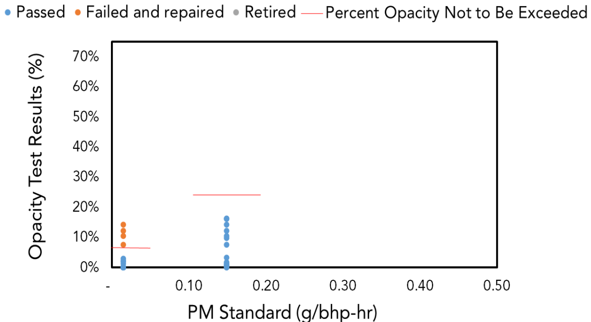
Figure E-23. RTG Opacity Test Results and PM standards
