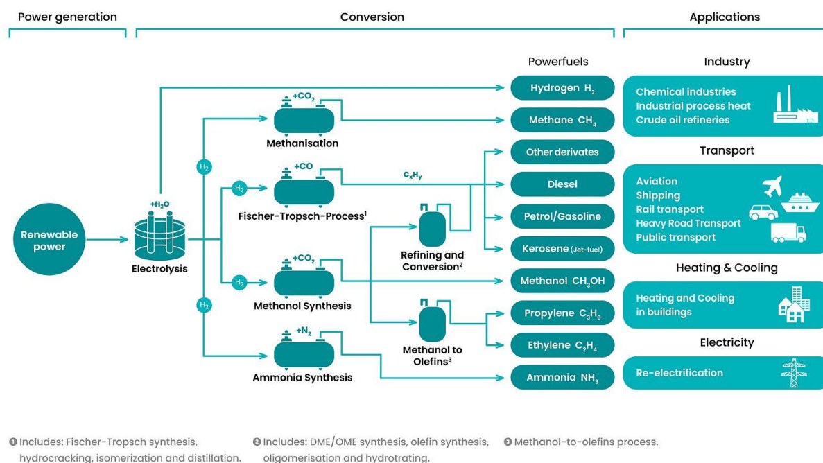
Figure 2. Production pathways of various power-to-liquid fuels ( Powerfuels – Global Alliance Powerfuels , 2022).
