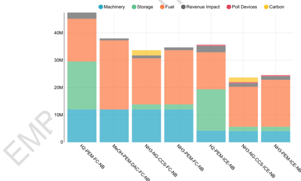
Figure 8.1 Total cost of ownership breakdown for fuel options in new-build shipping in 2030 (in USD)
