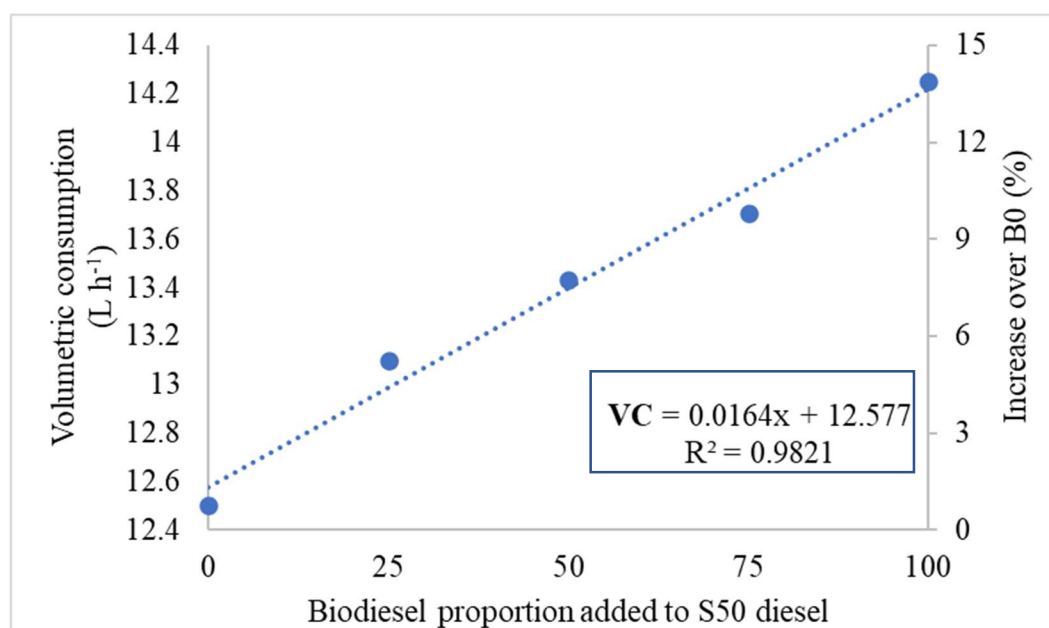
FIGURE 1. Volumetric fuel consumption as a function of biodiesel proportion.
