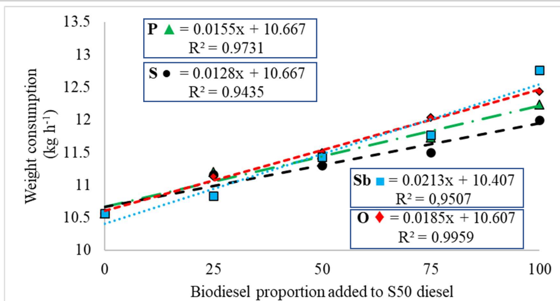
FIGURE 2. Weight fuel consumption of fuel as a function of the type and proportion of biodiesel.
