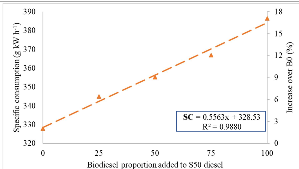
FIGURE 3. Specific fuel consumption as a function of the proportion factor.
