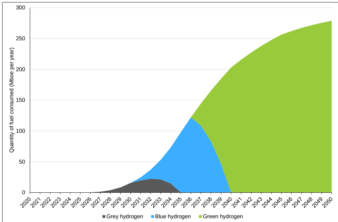
Figure 7-7: Split of hydrogen consumption under package 1 by grey, blue and green (million barrels of oil equivalent per year)
