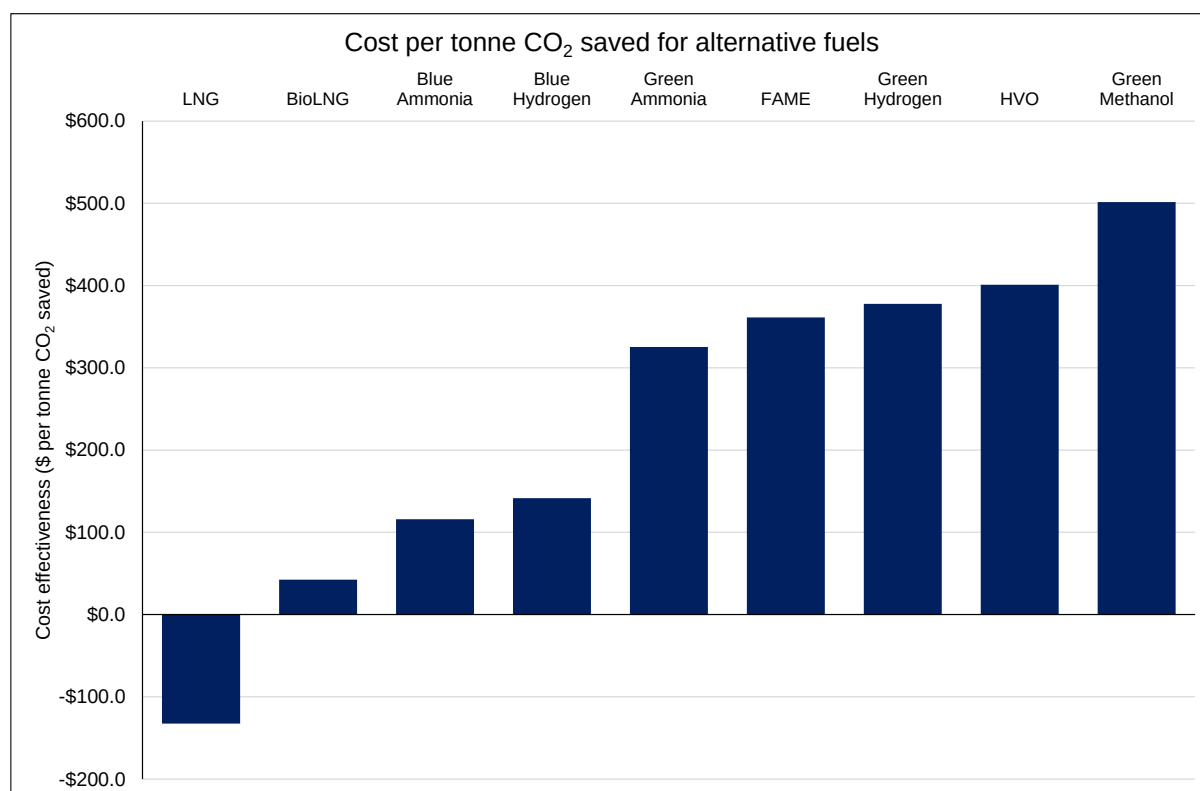
Figure 5-6: Cost-effectiveness ranking for alternative fuels
