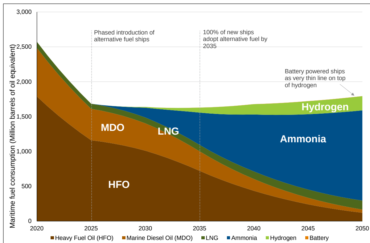
Figure 7-29: Fuel consumption to 2050 under the central scenario for Package 1A
