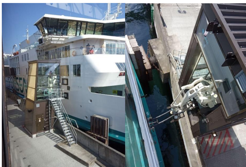
Figure 2: Shoreside 10.5 MW charging connection for Aurora af Helsingborg and Tycho Brahe passenger ferries.
