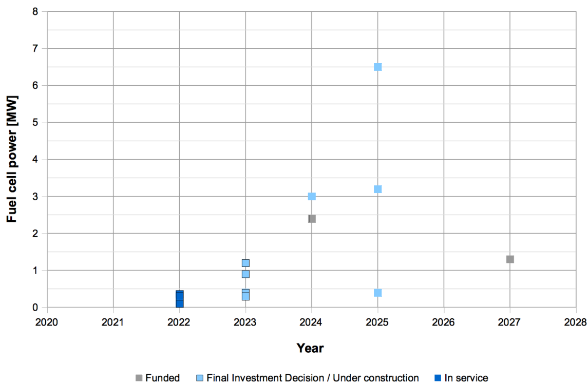
Figure 3: Installed fuel cell system nominal power outputs for existing and expected vessels.
