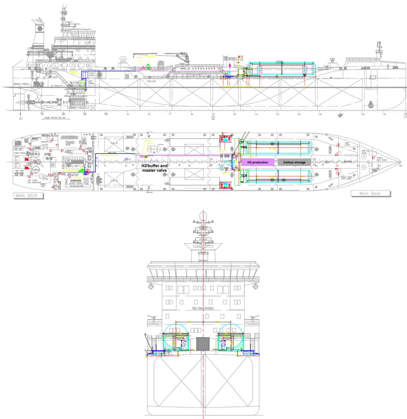
Figure 34. Chemical Carrier Application
