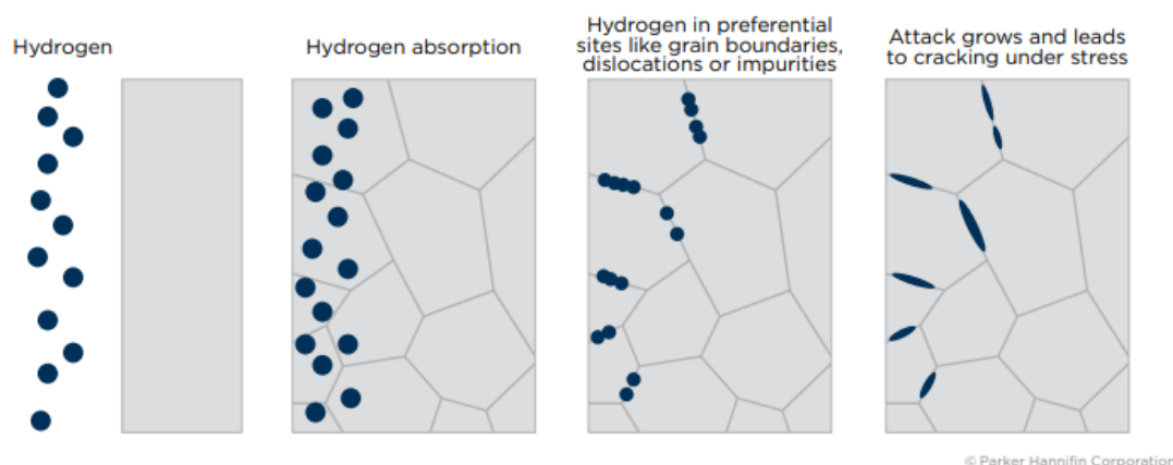
Figure 5. Illustration of hydrogen embrittlement (ABS, Sustainability Whitepaper, Hydrogen as Marine Fuel, 2021)
