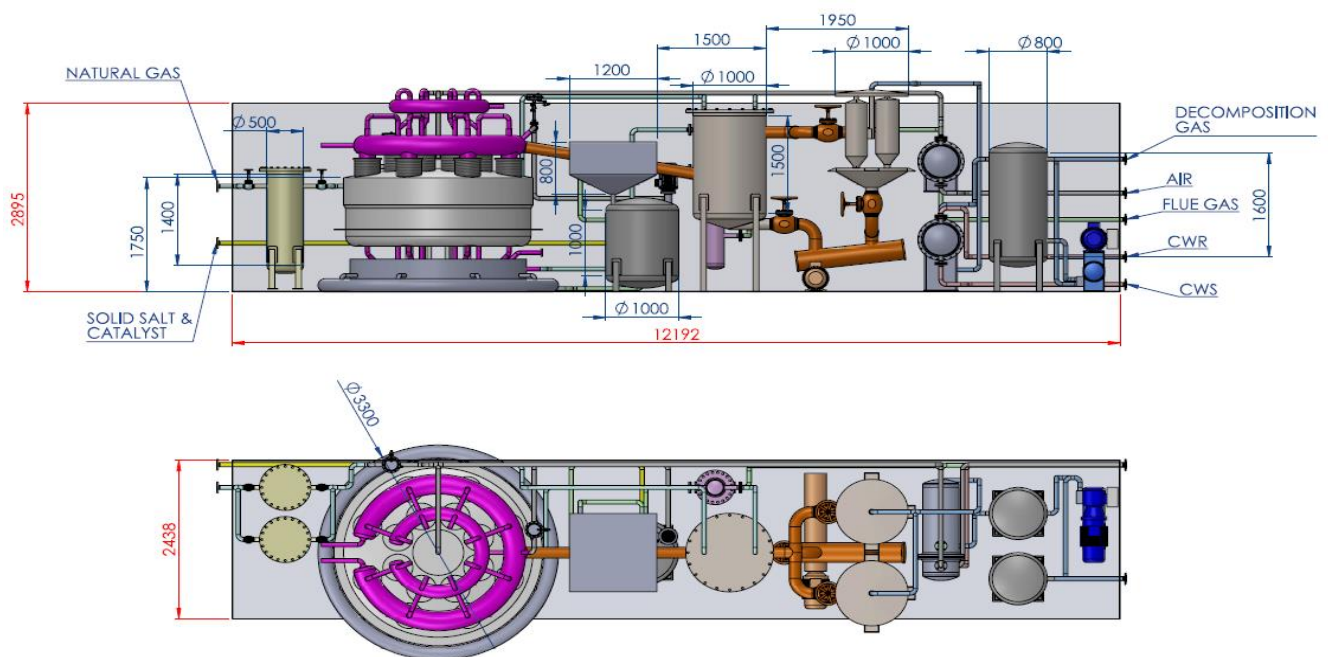
Figure 32. System General Arrangement
