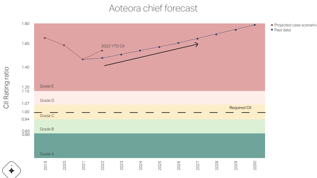
Figure 15: CII performance and projection.
