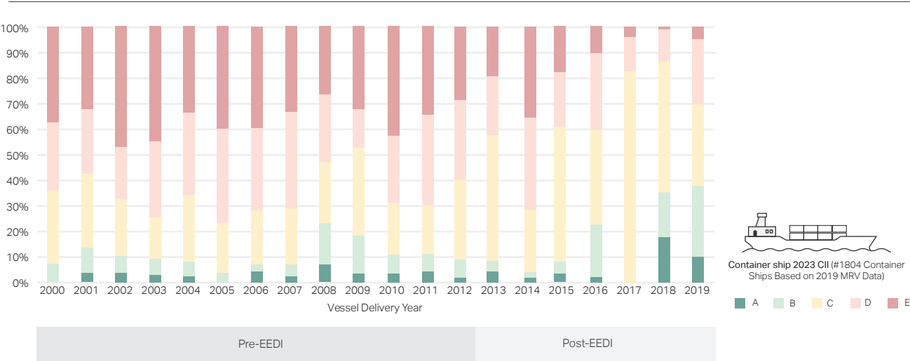
Figure 5: Cross-effects of the EEDI and CII – container vessels.
