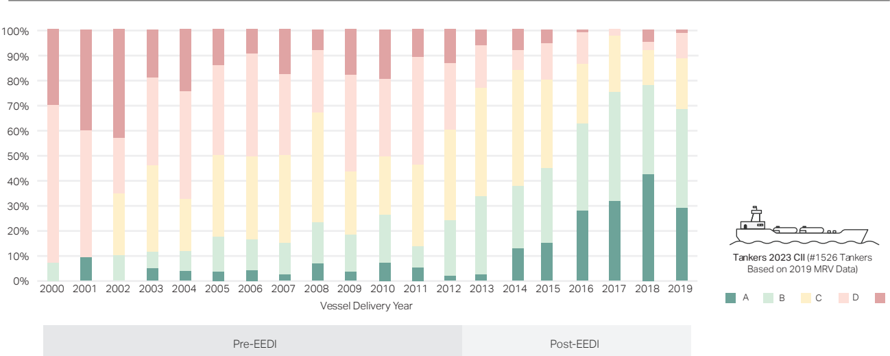
Figure 7: Cross-effects of the EEDI and CII – tankers.
