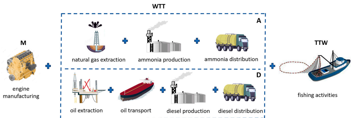
Figure 16. Processes included in the LCA of an ammonia-powered ship (ICE-A).
