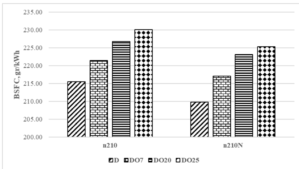
Figure 3 BSFC – Brake Specific Fuel Consumption for diesel fuel and biodiesel blends with different engine load conditions
