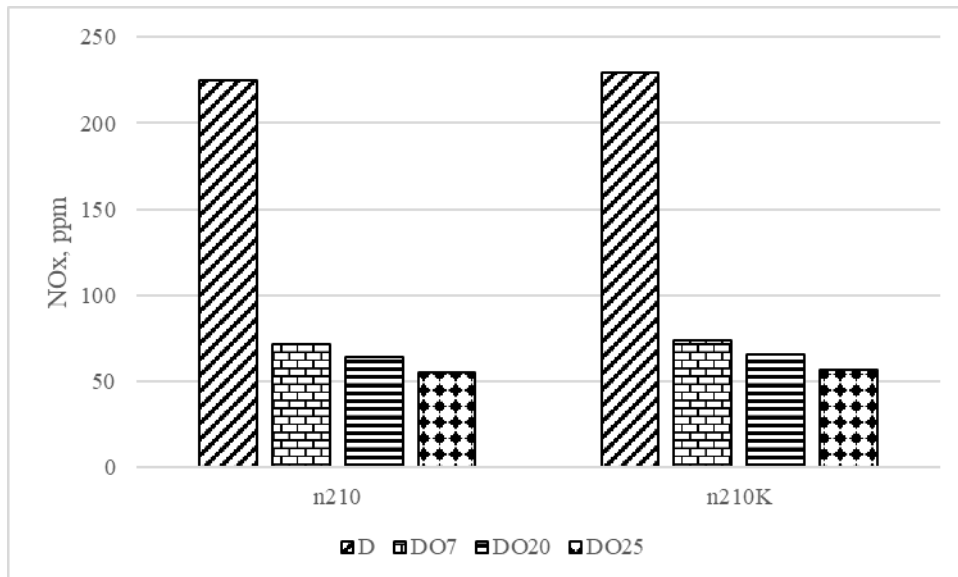
Figure 6 Exhaust emission of NO x for different fuels and engine loads, ppm
