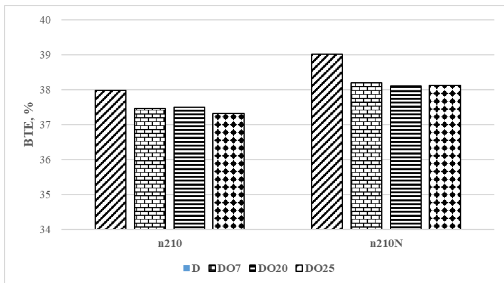
Figure 4 BTE – Brake Thermal Efficiency for diesel fuel and biodiesel blends with different engine load conditions
