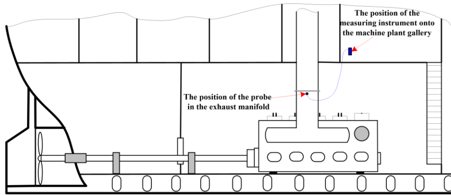
Figure 2 The position of exhaust emission testing equipment
