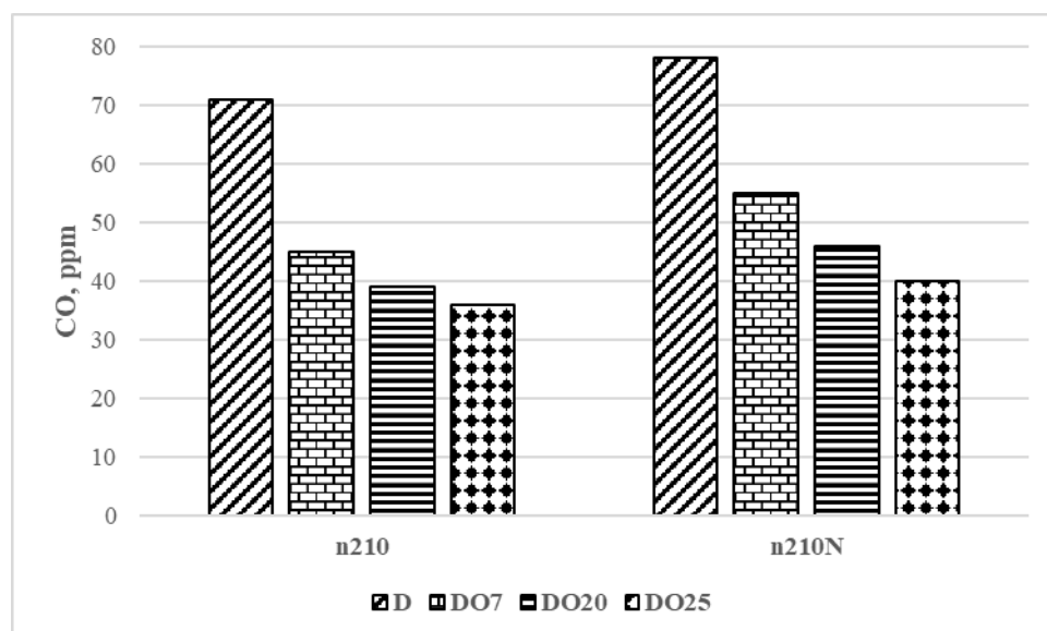
Figure 5 Exhaust emission of CO for different fuels and engine loads, ppm
