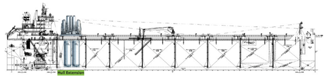
Fig. 17. Proposed arrangement for extending the length of the ship for accommodating for the captured \text{CO}_2 .
