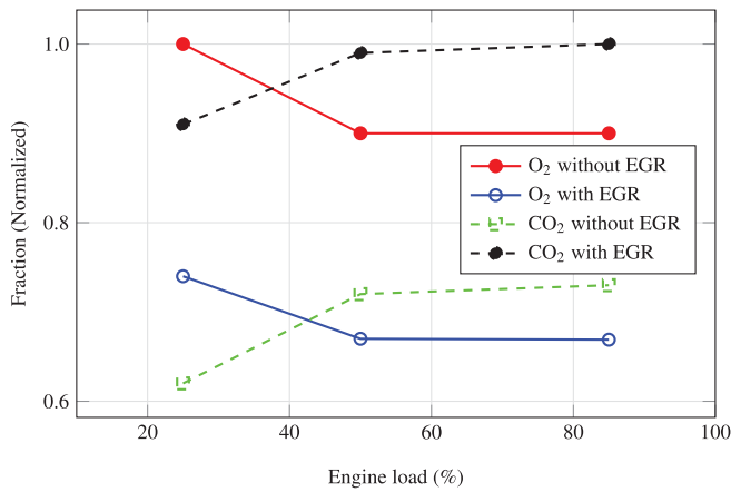
Fig. 16. Effect of EGR on \text{CO}_2 and \text{O}_2 on marine engine. The Y-axis has been normalized by the maximum mass fraction, which is in the load 85% for \text{CO}_2 and 25% for \text{O}_2 .
