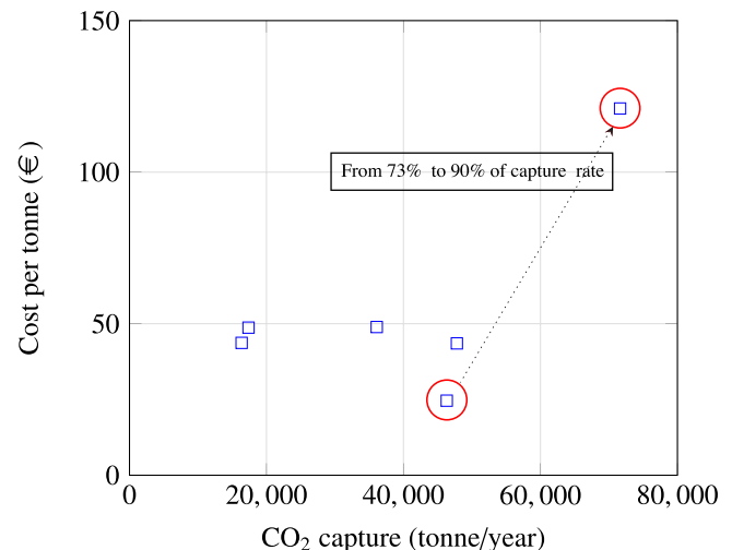
Fig. 3. The expected operational cost for installing carbon capture (Awoyomi et al., 2020, Luo and Wang, 2017, Ros et al., 2022).
