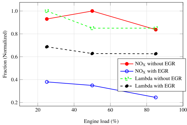
Fig. 15. Effect of EGR on lambda and \text{NO}_x emission on marine engine. The Y-axis has been normalized by the maximum mass fraction, which is in load 50% for \text{NO}_x and 25% for lambda.
