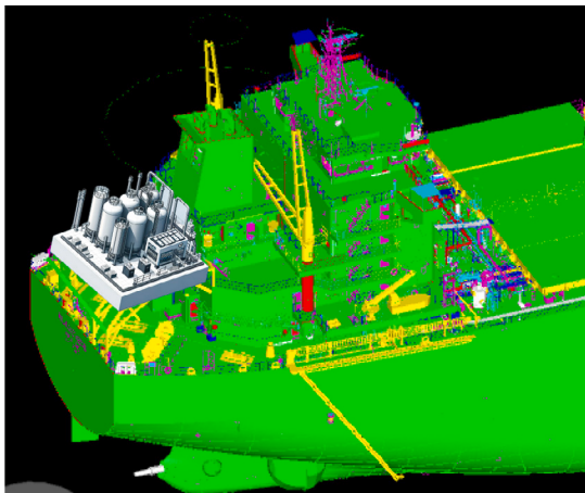
Fig. 7. An arrangement for the high columns and all the machinery in the extension of accommodation deck.
