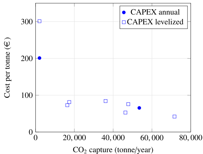
Fig. 2. Capital cost of onboard carbon capture reported by several studies. 1 The much higher cost at a low CO 2 capture included the labor, maintenance and use of chemicals (Monteiro, 2020, Ros et al., 2022, Luo and Wang, 2017, Güler and Ergin, 2021, Awoyomi et al., 2020, Oh et al., 2024).
