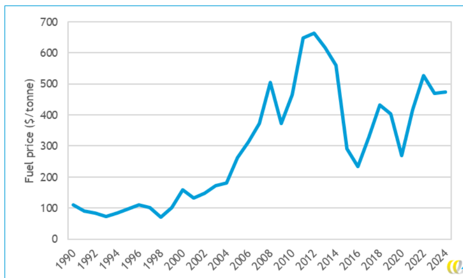
Figure 3 - Average yearly fuel prices (HSFO 380cst Bunker Prices (3.5% Sulphur), Singapore), 1990-2024
