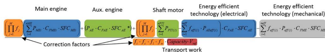
Figure 2 - EEDI formula
