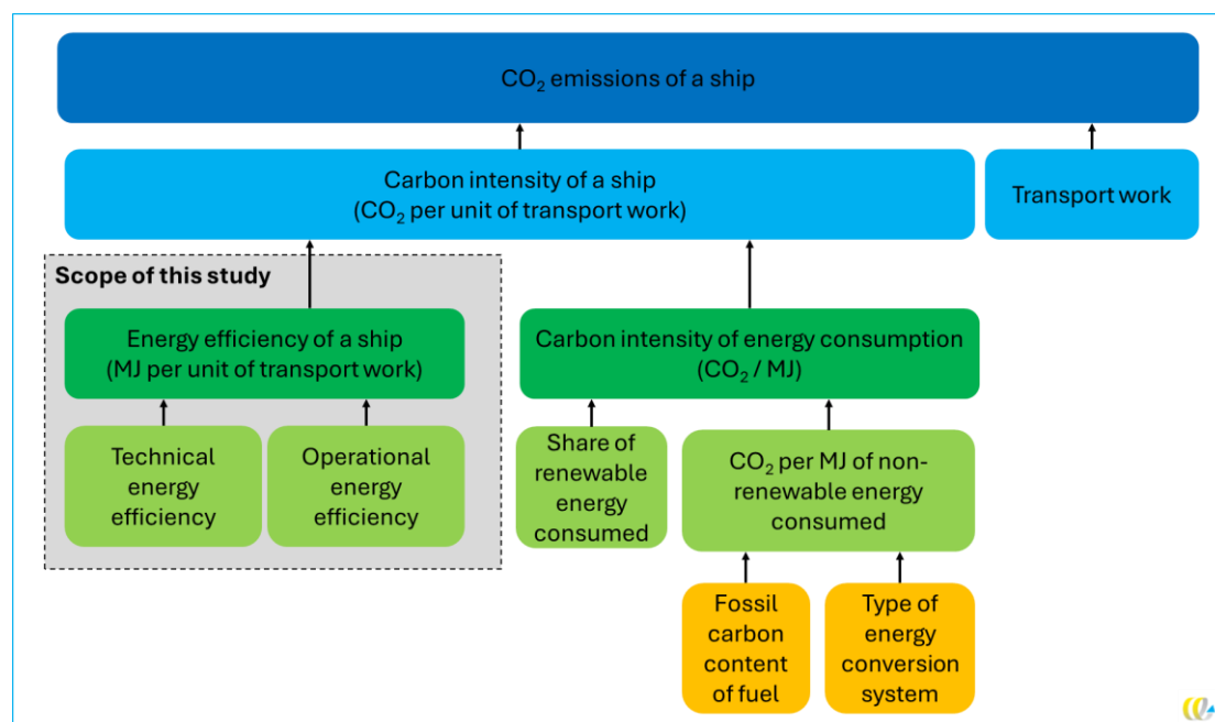
Figure 1 - Determinants of CO 2 emissions, carbon intensity and energy efficiency of maritime transport
