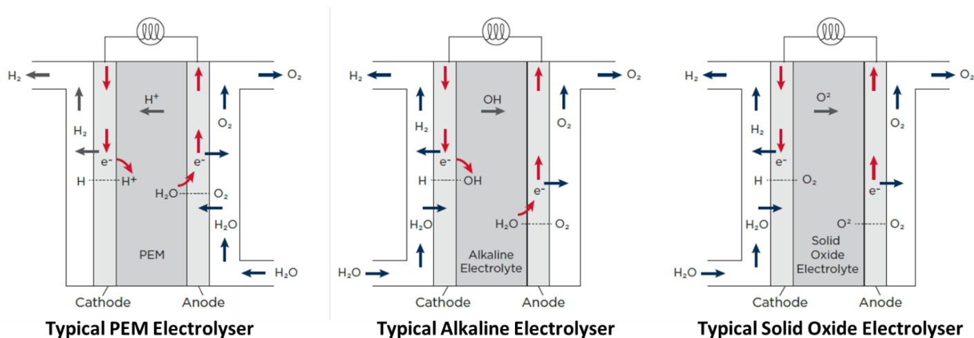
Figure 3. Electrolyser technologies currently available or under development (ABS).
