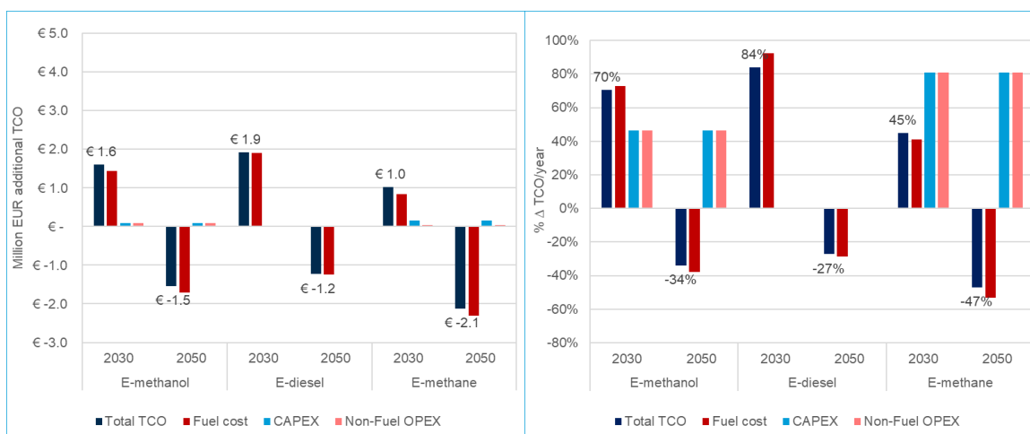
Figure 9. Annual difference in TCO of e-fuel-powered bulk ships (35,000-60,000 DWT).
