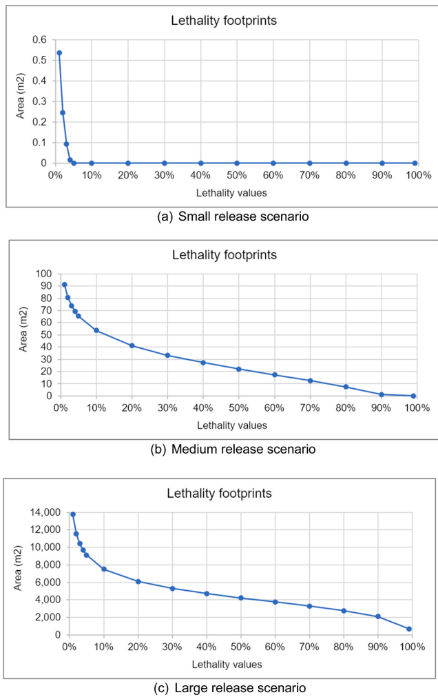
Fig. 3. The area of lethality footprints in the baseline scenarios.
