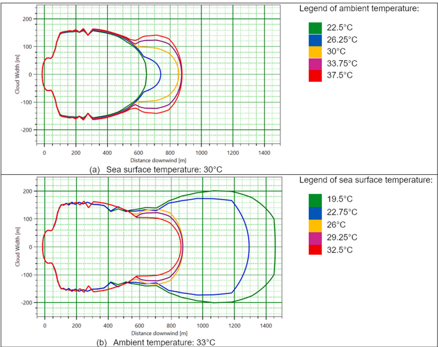
Fig. 9. The effect of air temperature and sea surface temperature on the 1100 ppm maximum cloud footprint in large release scenarios.
