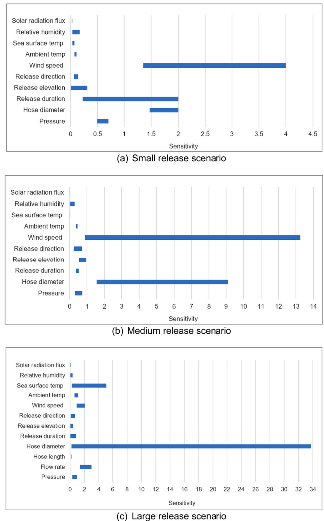
Fig. 4. Sensitivities of different factors to 1100 ppm maximum cloud footprint.
