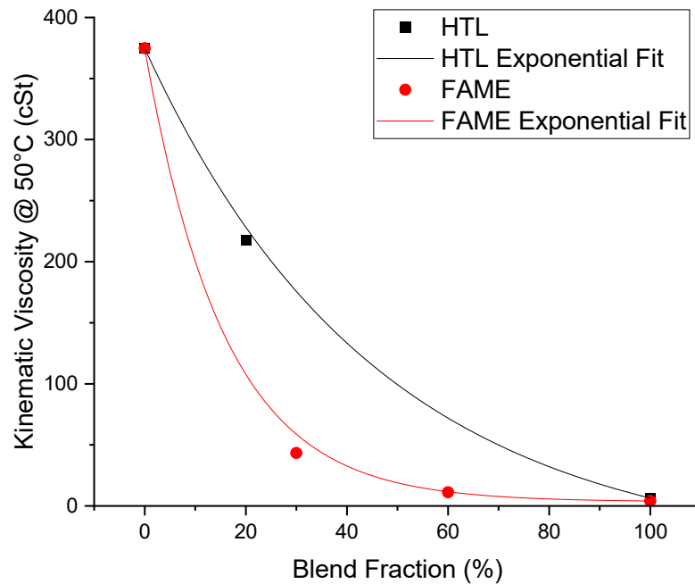
Figure 5. Viscosity blending effects of HTL and FAME biofuels with VLSFO
