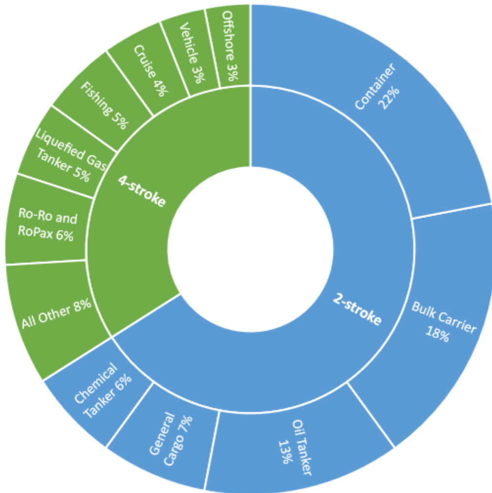
Figure 2. Fuel consumption by ship main engine type. Data from Concawe [7].
