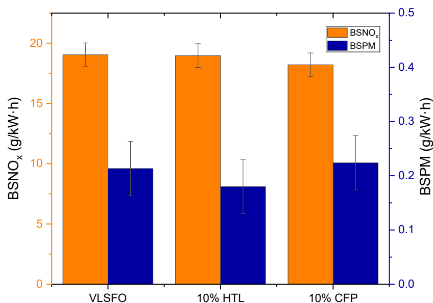
Figure 7. Brake-specific NO x (BSNO x ) and brake-specific PM (BSPM) emissions at high-speed, high-load operation for VLSFO and 10% blends of HTL and CFP fuels in the Enterprise research engine. Error bars represent the standard deviation of 8 repeats of the baseline VLSFO fuel.
