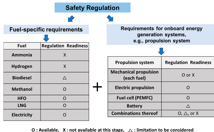
Figure 6. Flow chart for evaluation of safety regulation readiness.
