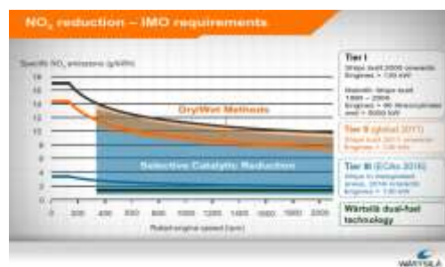
Figure 1. NO x Relationship – Engine Speed (Wartsila 20 Dual Fuel (DF) Engine Presentation, 2010)
