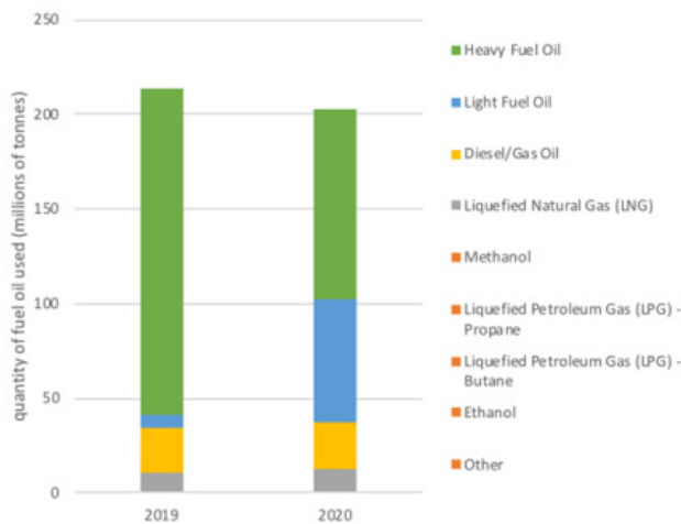
Figure 4. Fuel Oil consumption of Ships [64]
