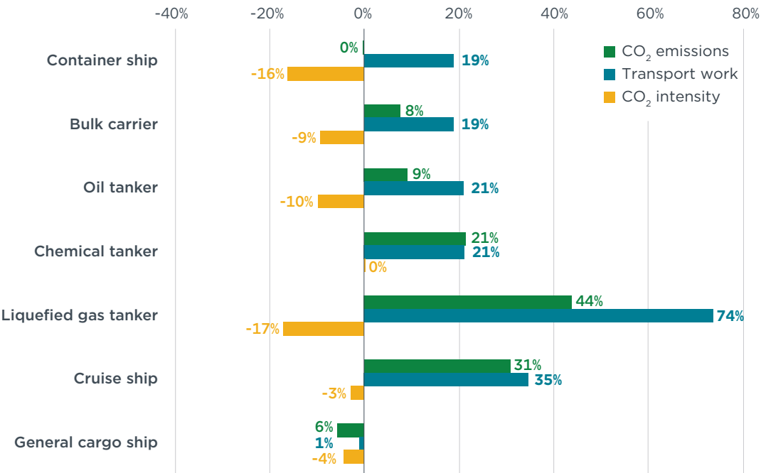
Figure 12 Change in transport work, fleet-wide carbon intensity, and total CO 2 emissions in 2023 compared with 2016 for the seven highest-emitting ship classes
