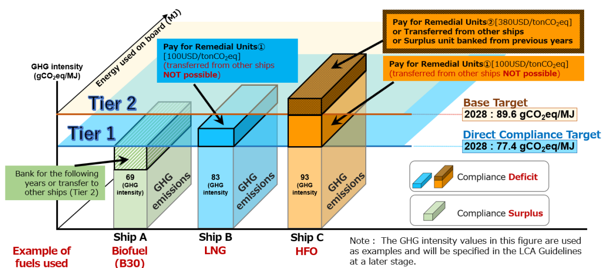
Examples of GFI compliance approaches based on GHG intensity of ships
