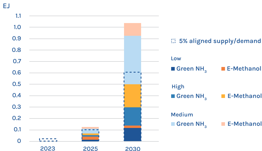
Figure 4. Estimated total supply from SZE for maritime usage compared to 0.6 EJ 2030 requirement in line with the 5% SZE 2030 goal. 20
